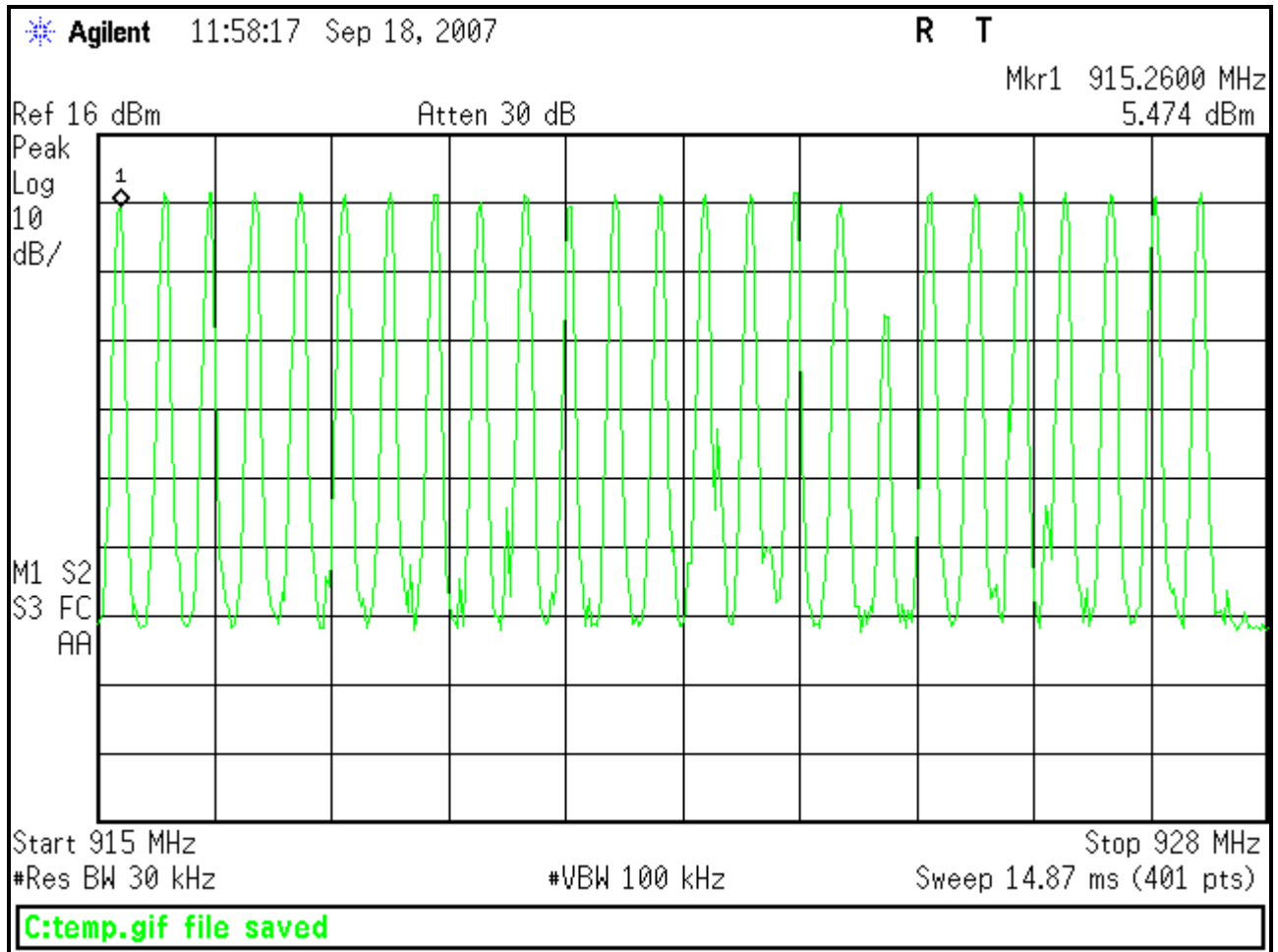
25 Channel Hopping Frequencies from 915 to 928 MHz
