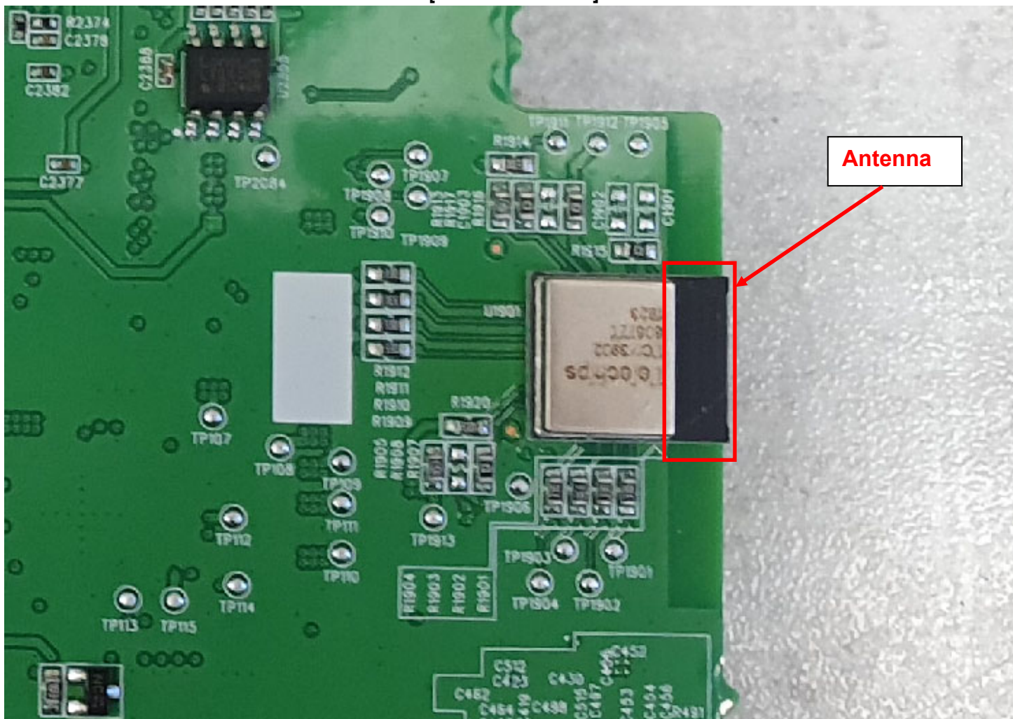
[Bluetooth Module]
