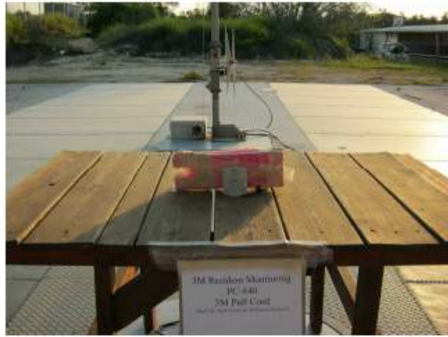
Figure 4. Radiated Emission Test 30MHz-4500MHz
