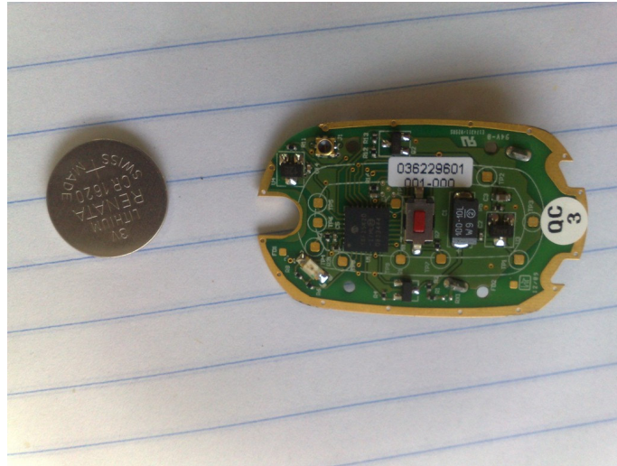
Figure 3: PB-830 PCB (Bottom)
