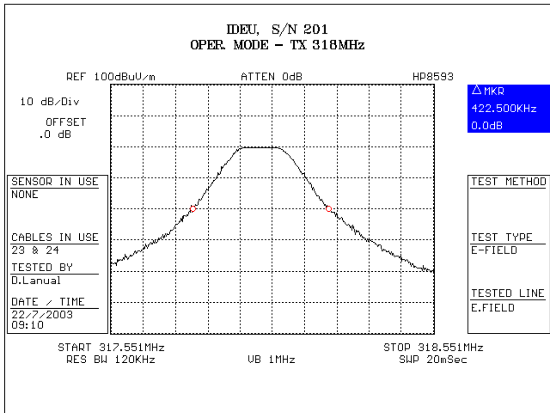
Plot 13. 1 Bandwidth
