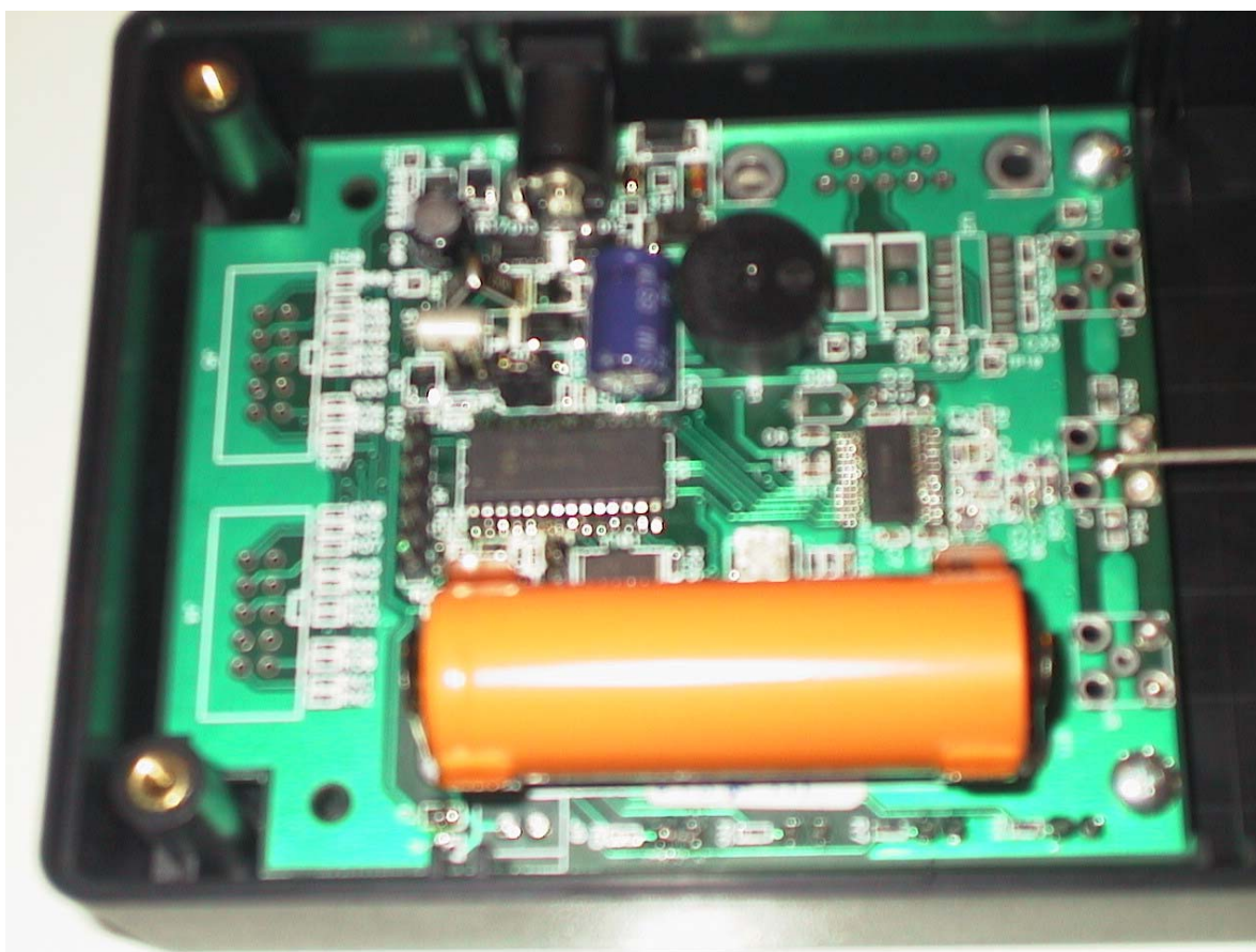
Picture 14.6 EUT
