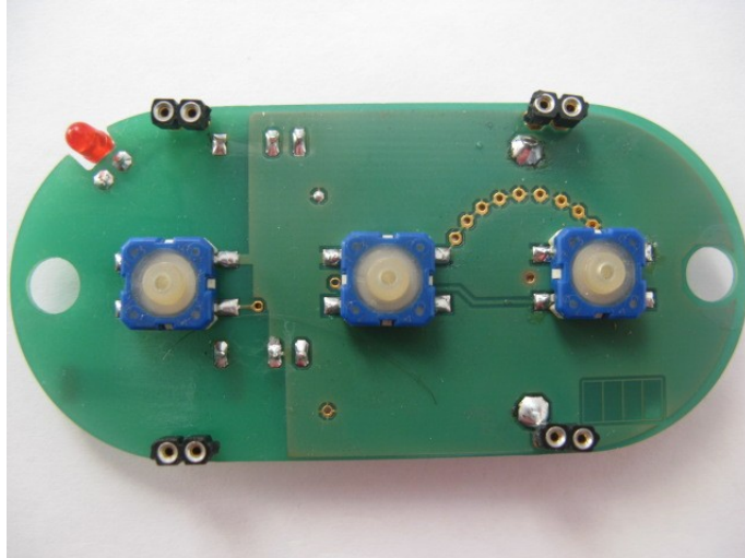
FRONT SIDE VIEW WITH TX MODULE
