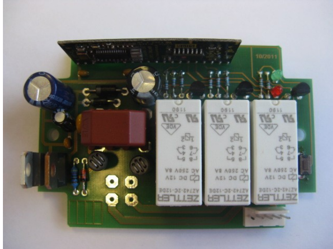
RX FRONT WITH RX MODULE
