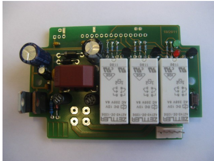
RX FRONT VIEW
