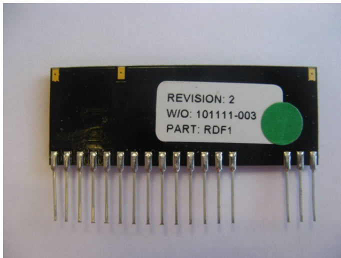
RX MODULE – REAR VIEW
