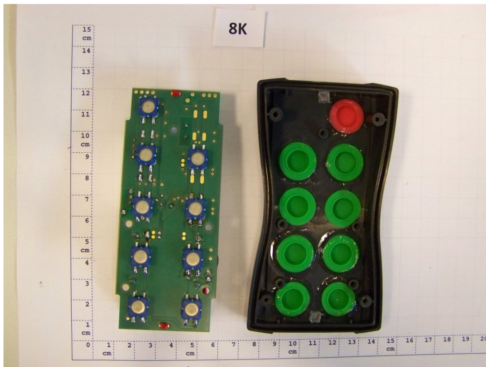
Photograph 6: PCB layout removed rear side of EUT C with cover(right)
