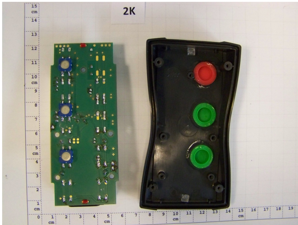
Photograph 5: PCB layout removed rear side of EUT A with cover(right)
