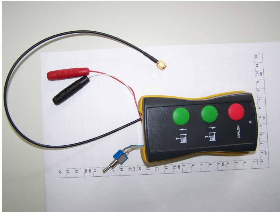
Photograph 3: EUT B used for conducted tests
