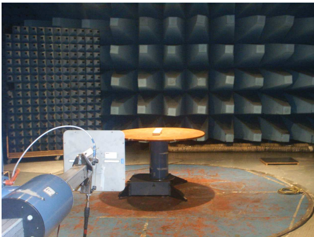
Radiated emission 1000 MHz to 5000 MHz
