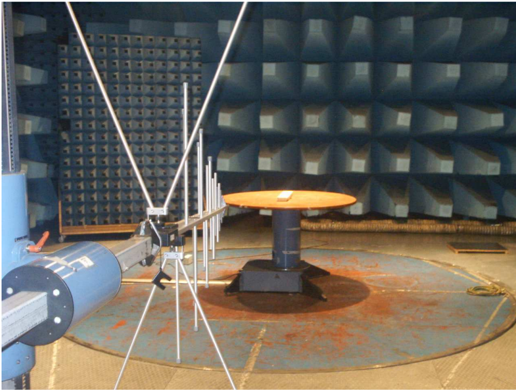
Radiated emission 30 MHz to 1000 MHz
