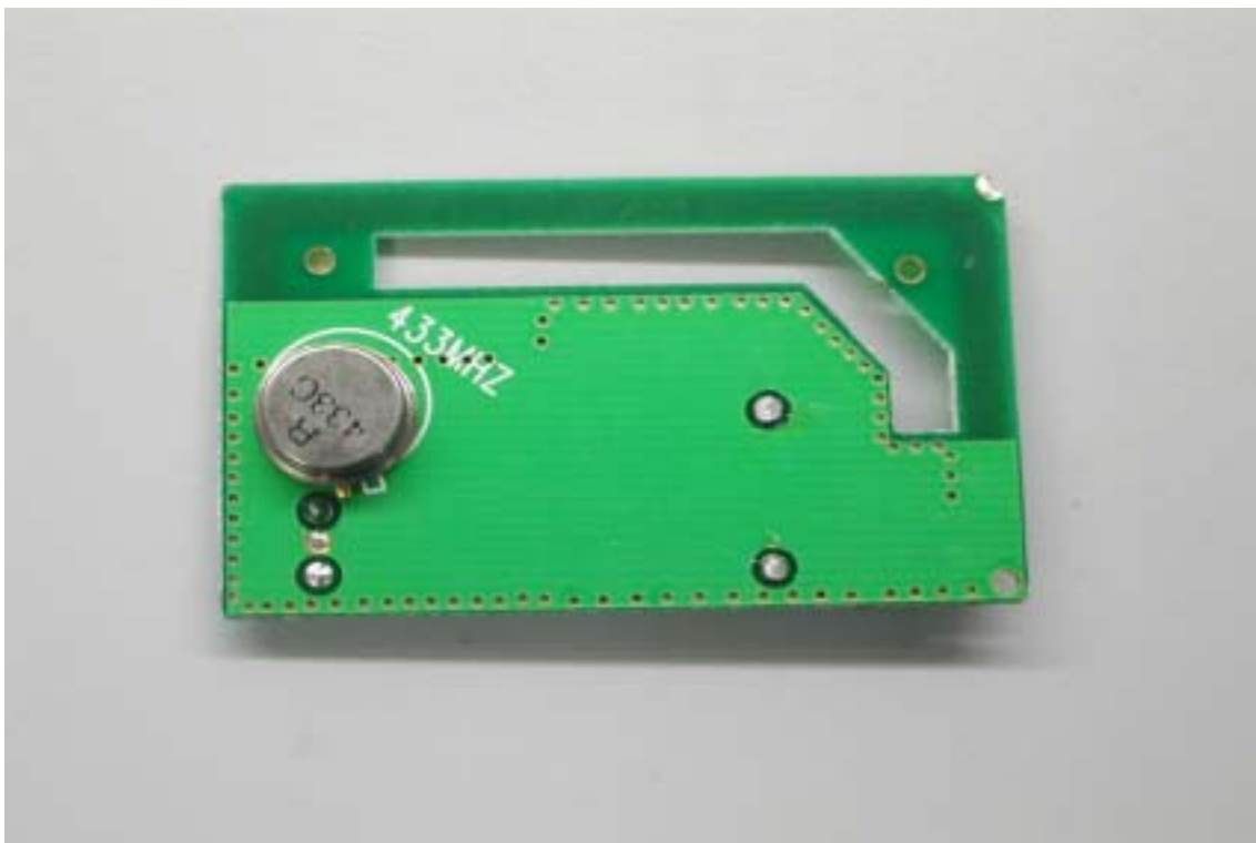
Internal of EUT (RF Module) – 5
