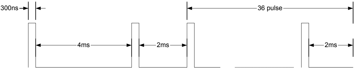
Long pulse Train Length=87.1ms
