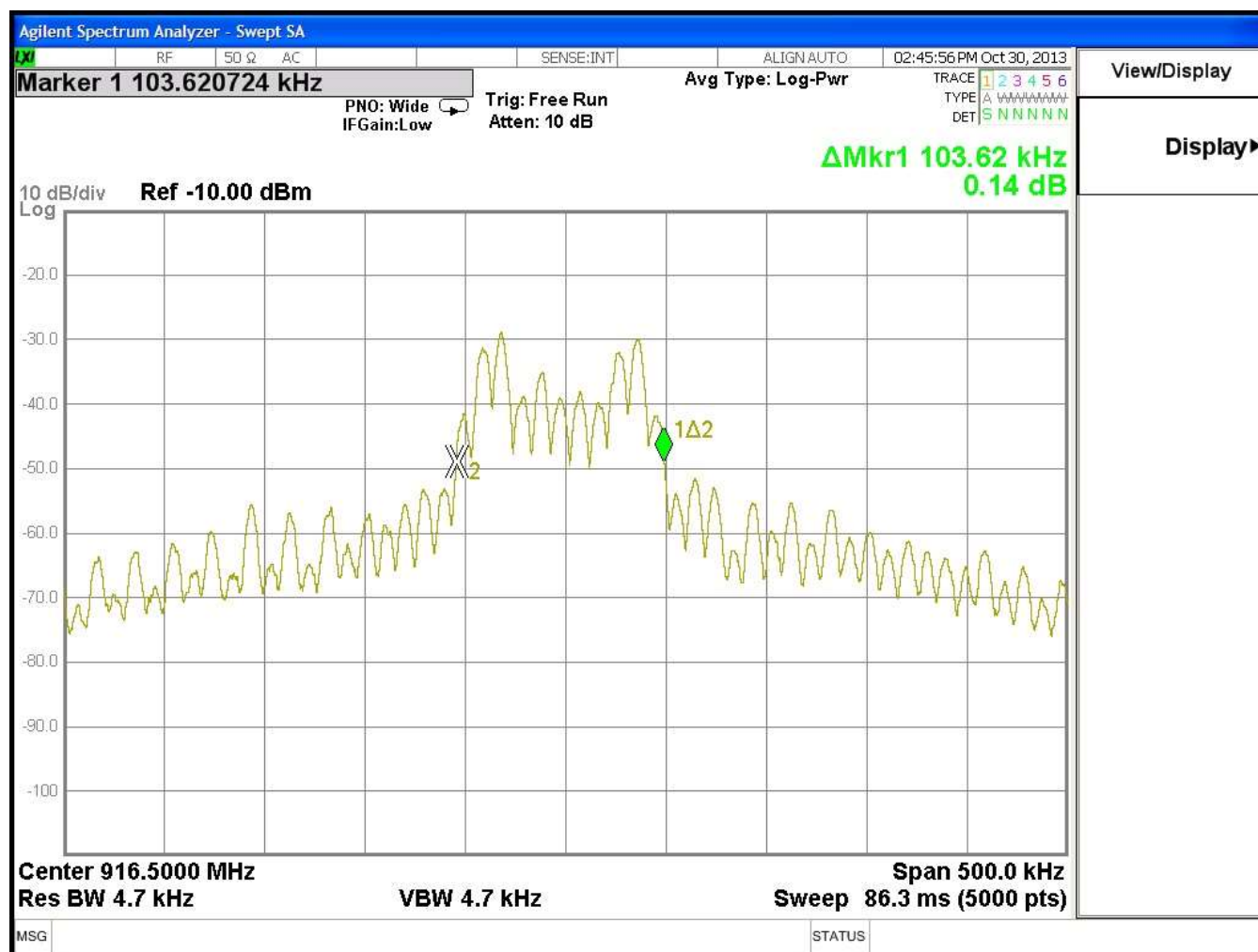
Figure 6: Occupied Bandwidth
