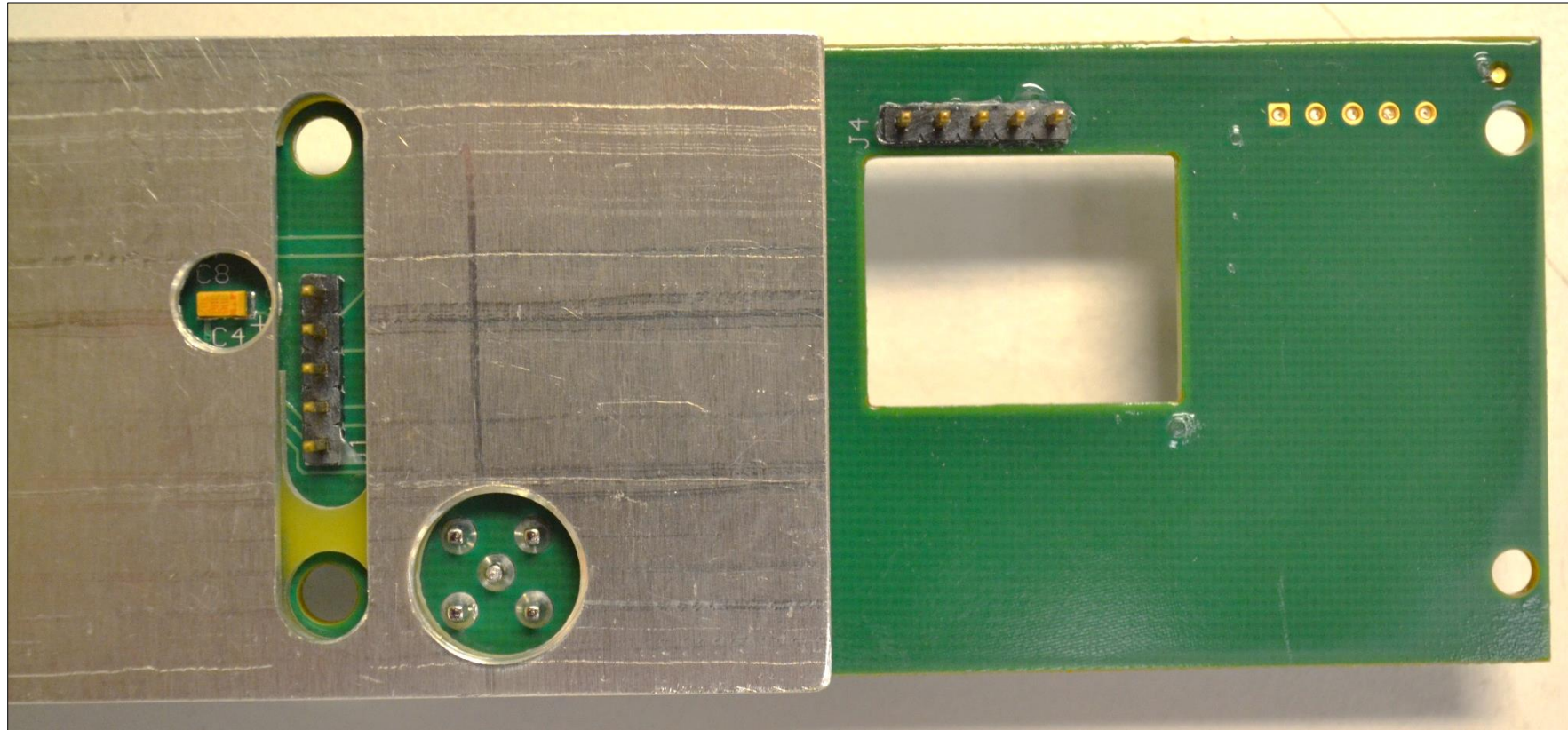
Magnetic Field Generator w/ CAM -Internal Photo CAM Board-Bottom View (pt. 2-with spacer)
