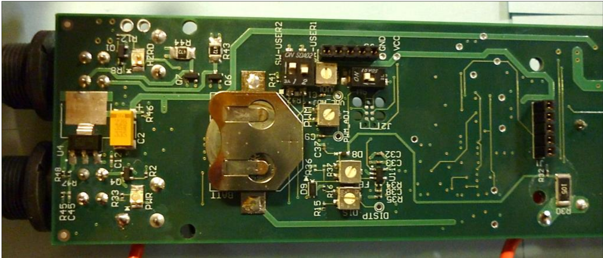
Magnetic Field Generator w/ CAM -Internal Photo Generator/Receiver Board-Bottom View (pt. 2)
