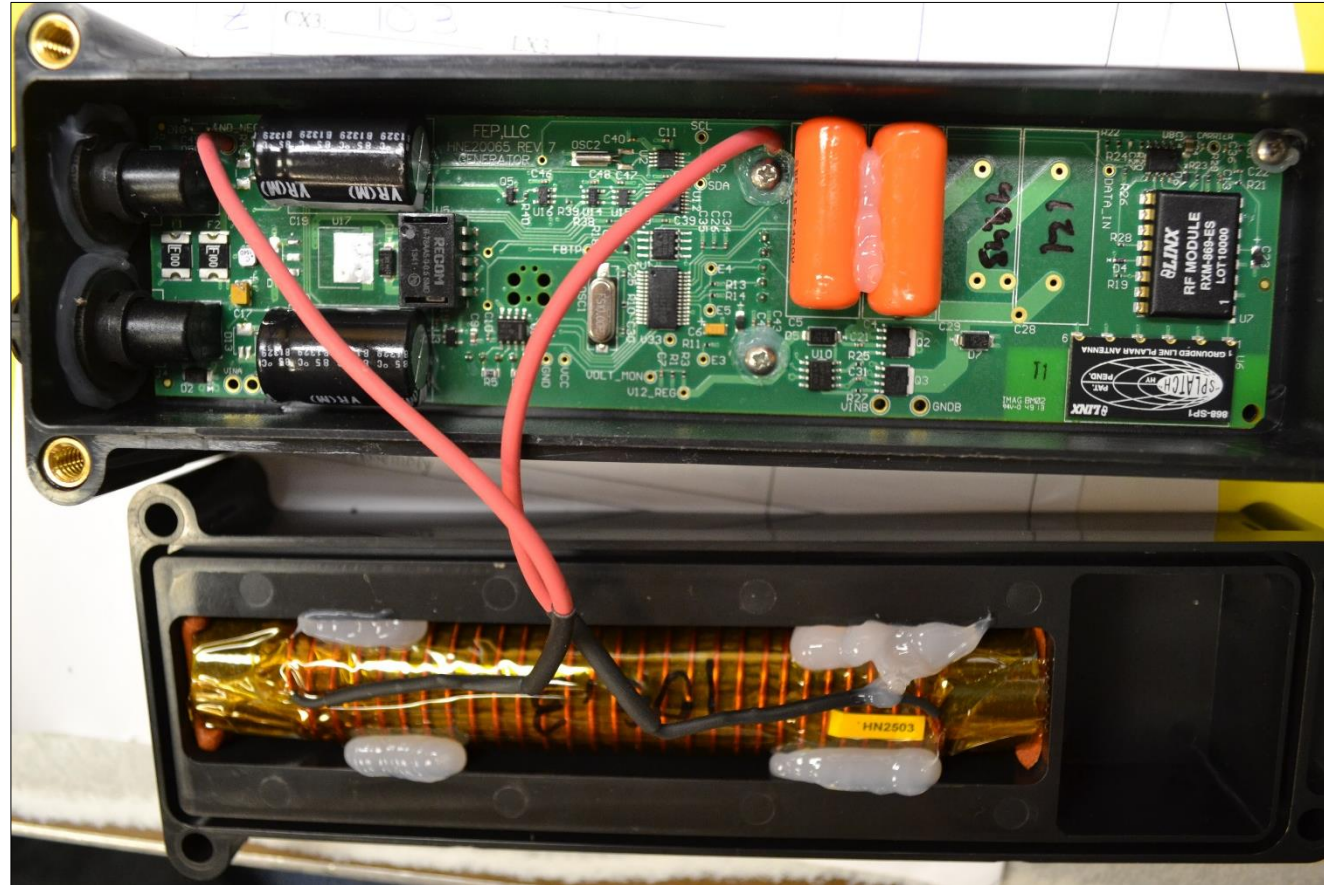
Magnetic Field Generator w/ CAM -Internal Photo Open Ferrite and Middle Housings Circuitry and Wire/Inductor
