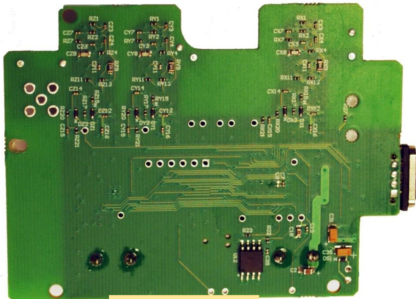
Printed Circuit Board-Back Side
