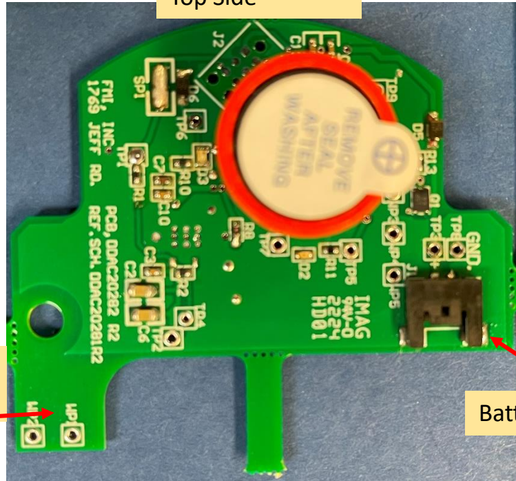
Charger Board- Top Side
