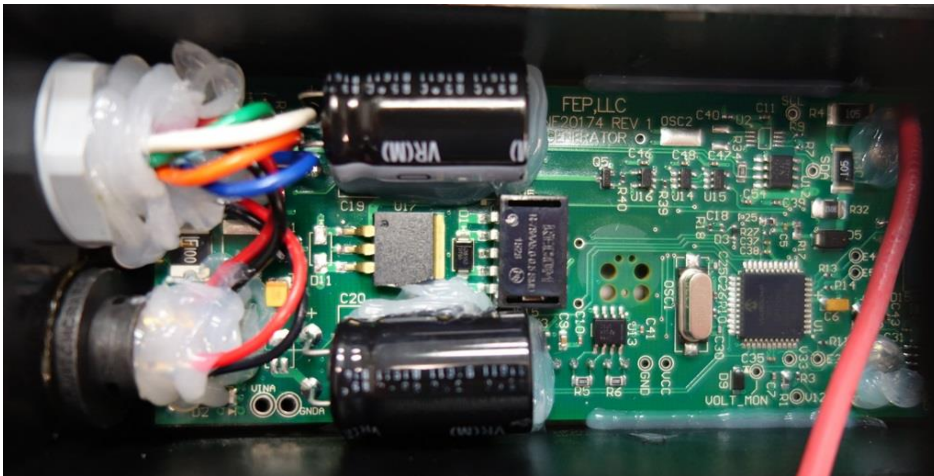
Magnetic Field Generator w/ CAM -Internal Photo Generator/Receiver Board-Top View (pt. 2)
