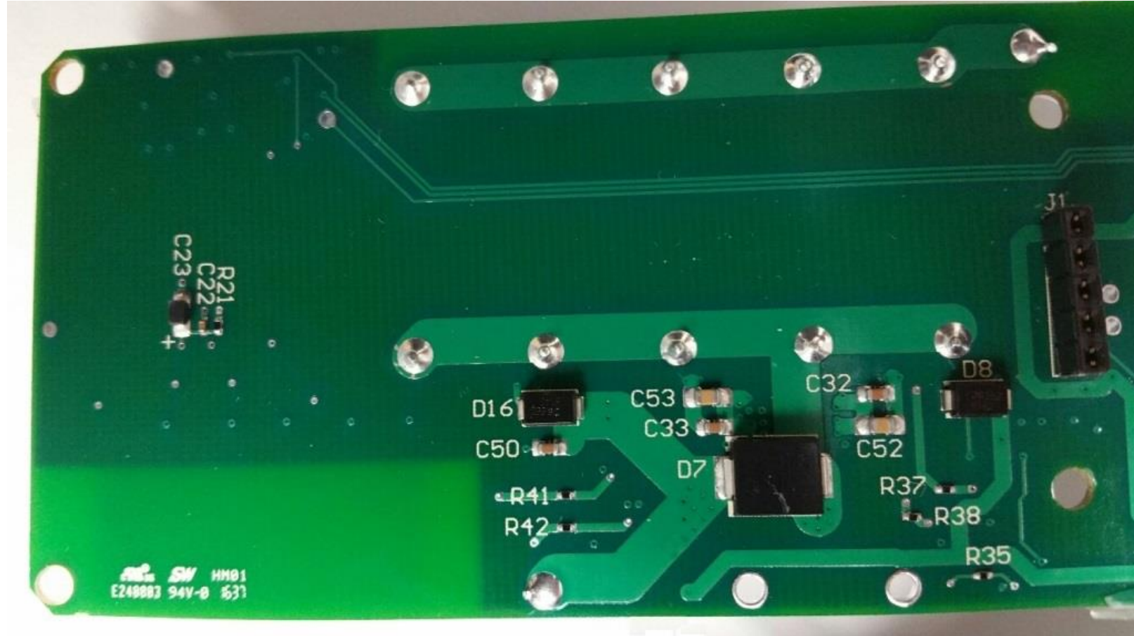
Magnetic Field Generator w/ CAM -Internal Photo Generator/Receiver Board-Bottom View (pt. 1)
