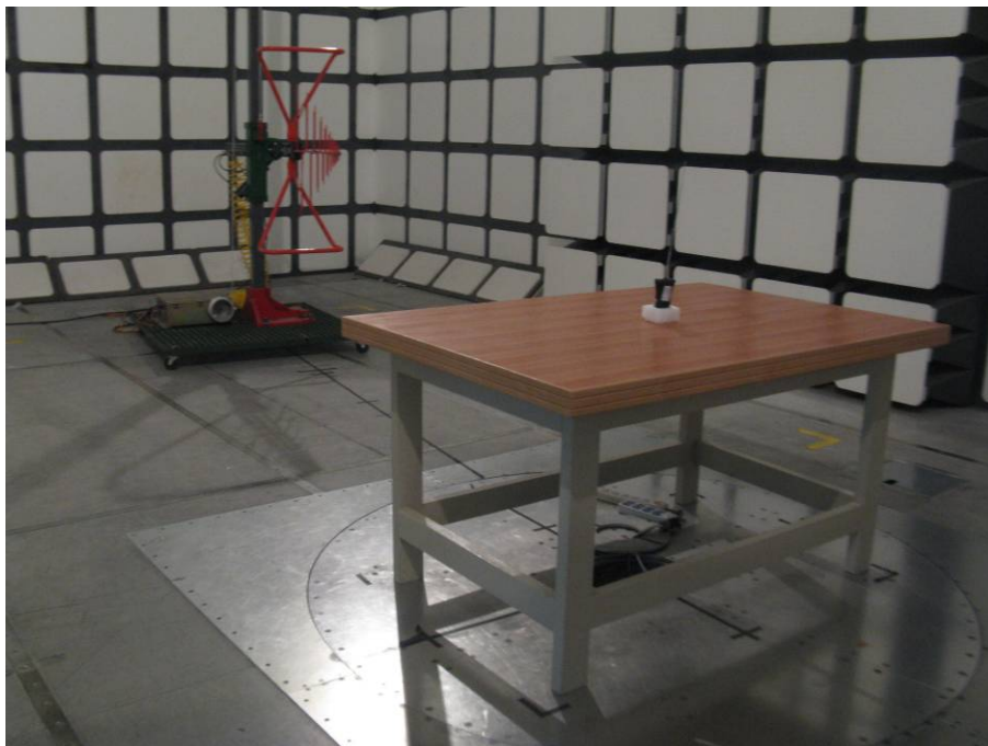
Radiated Emissions – Stand Rear View (30MHz-1GHz)
