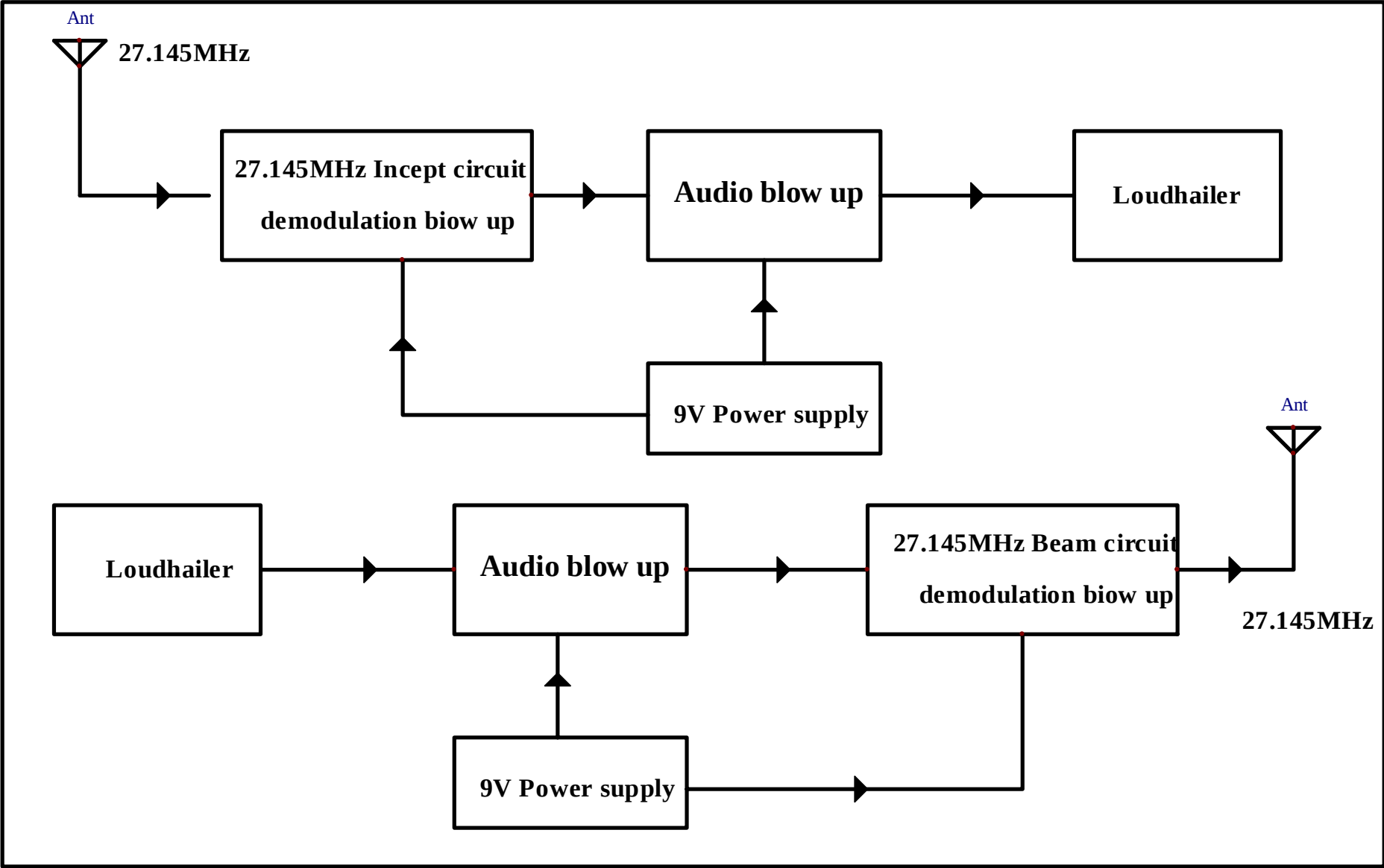
Intercom Walkie Talkie ZR33120C Block Diagram
