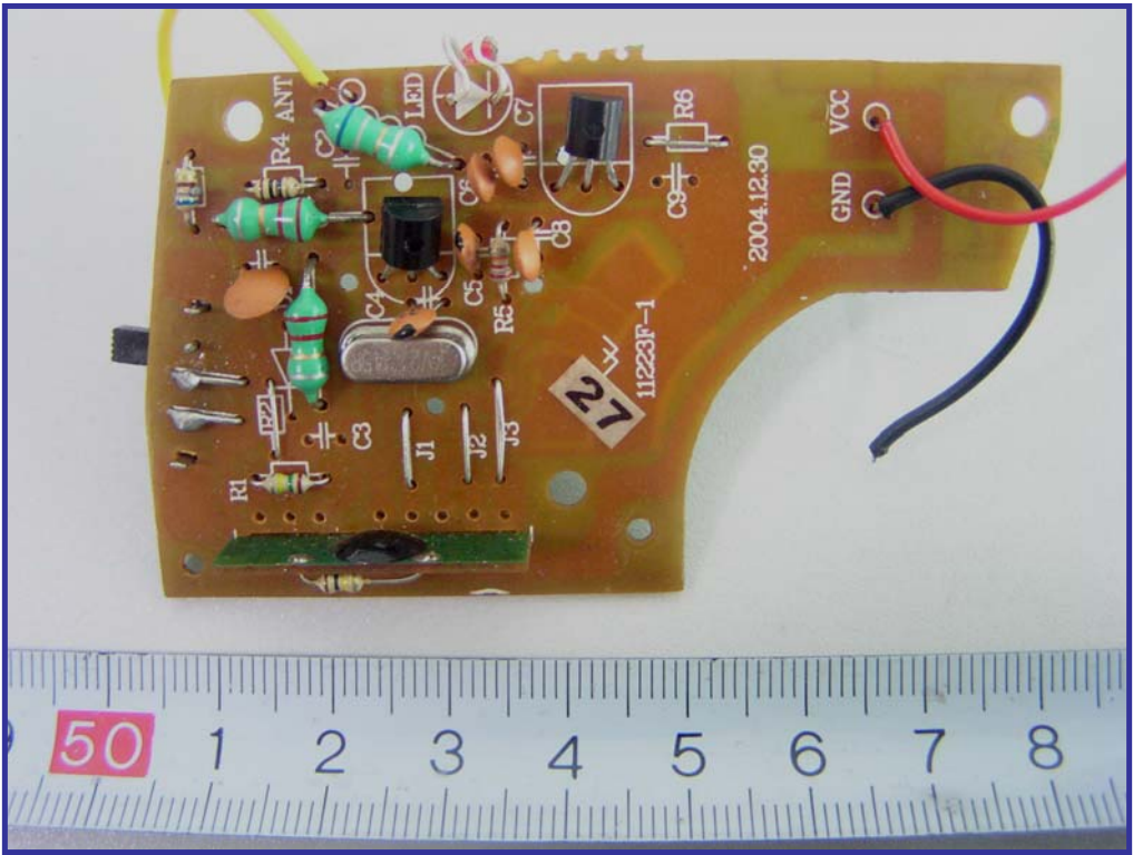
EUT - Board Component View
