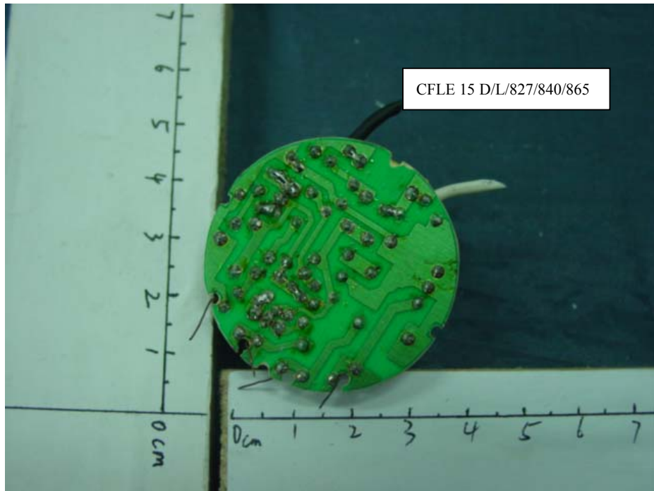
FIGURE 13 Energy Saving Lamp Main Board (Soldered Side)
