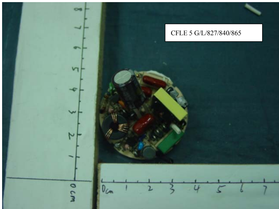
FIGURE 22 Energy Saving Lamp Main Board (Component Side)
