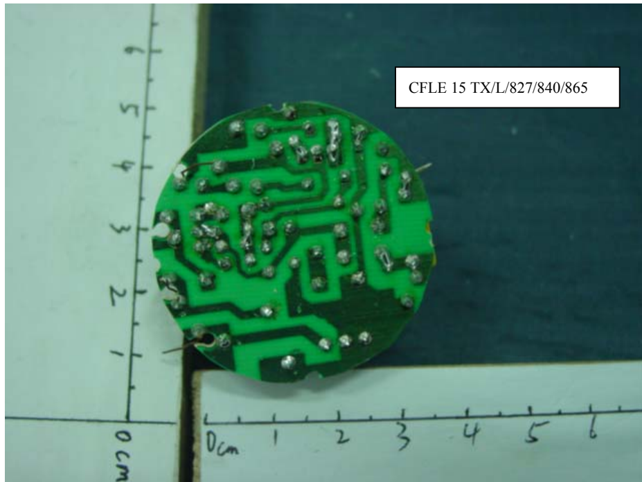
FIGURE 21 Energy Saving Lamp Main Board (Soldered Side)
