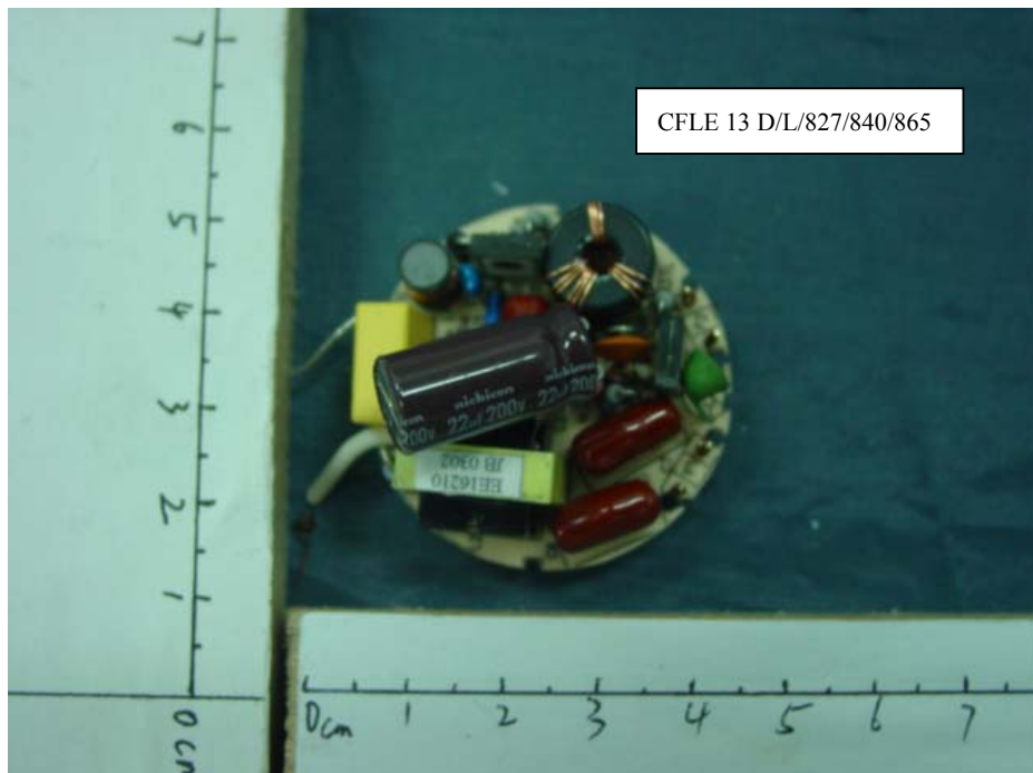
FIGURE 10 Energy Saving Lamp Main Board (Component Side)
