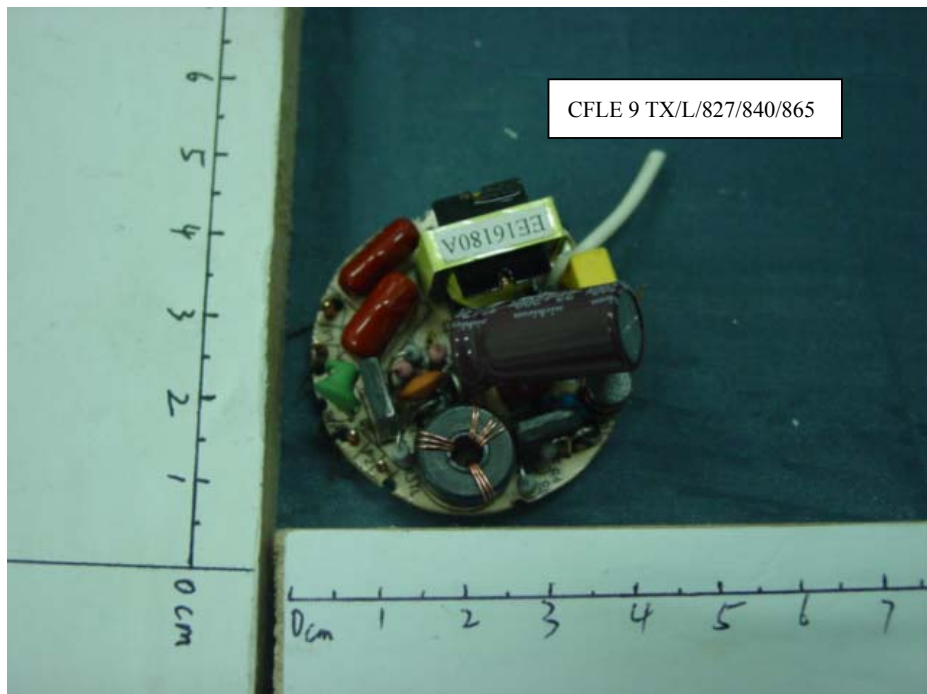
FIGURE 14 Energy Saving Lamp Main Board (Component Side)
