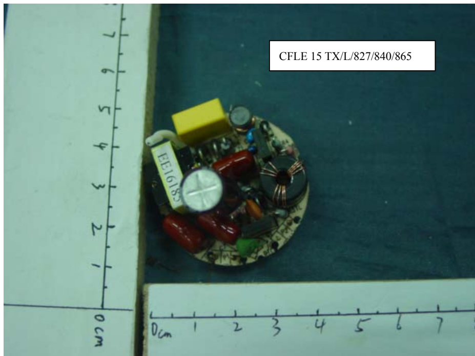
FIGURE 20 Energy Saving Lamp Main Board (Component Side)
