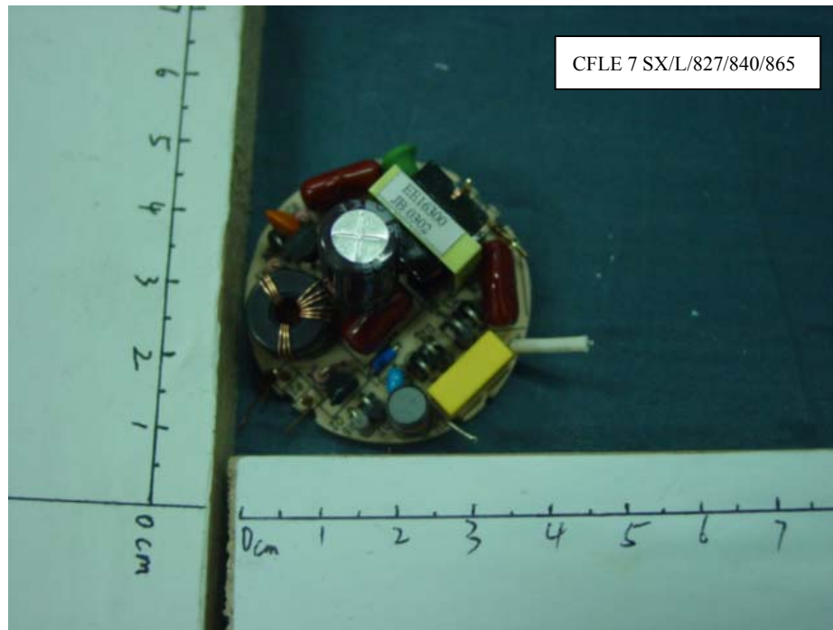
FIGURE 5 Energy Saving Lamp Main Board (Component Side)
