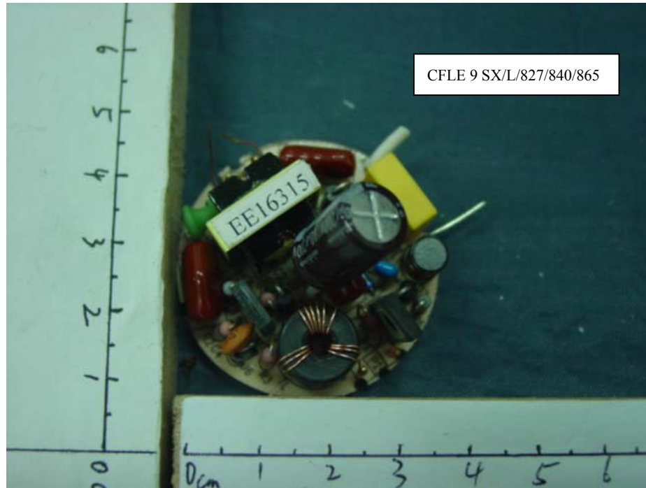
FIGURE 7 Energy Saving Lamp Main Board (Component Side)
