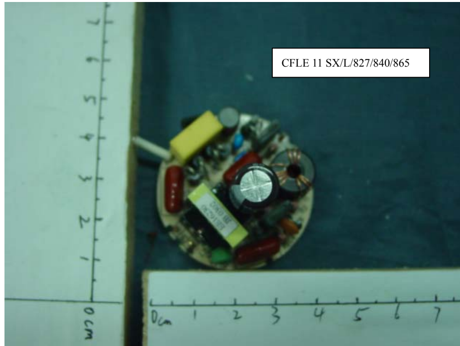
FIGURE 9 Energy Saving Lamp Main Board (Component Side)
