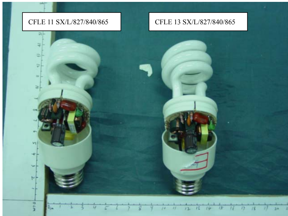
FIGURE 2 Energy Saving Lamp Cover Removed
