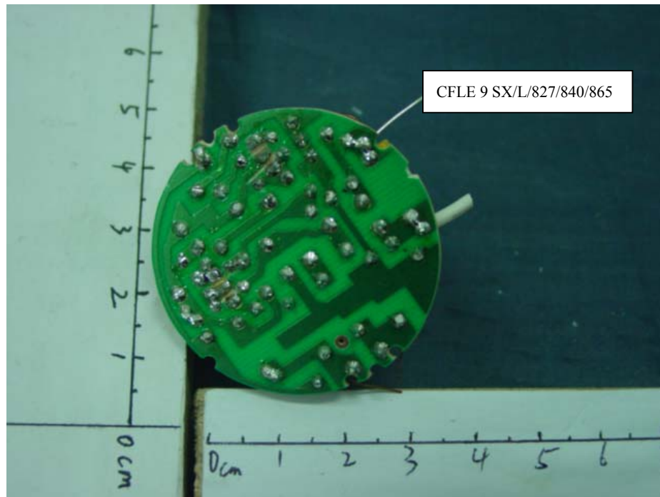
FIGURE 8 Energy Saving Lamp Main Board (Soldered Side)
