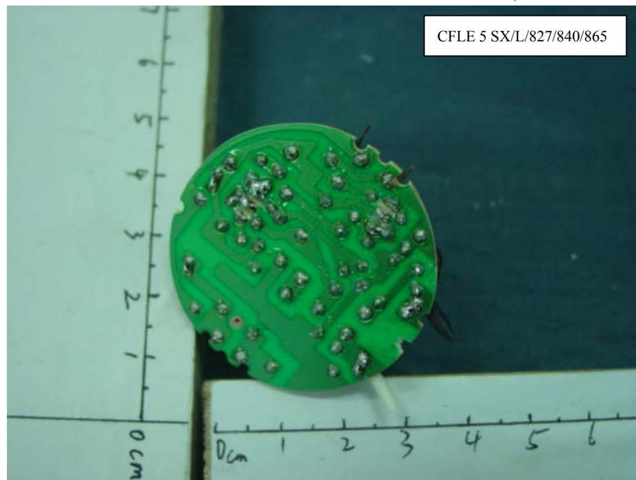
FIGURE 4 Energy Saving Lamp Main Board (Soldered Side)
