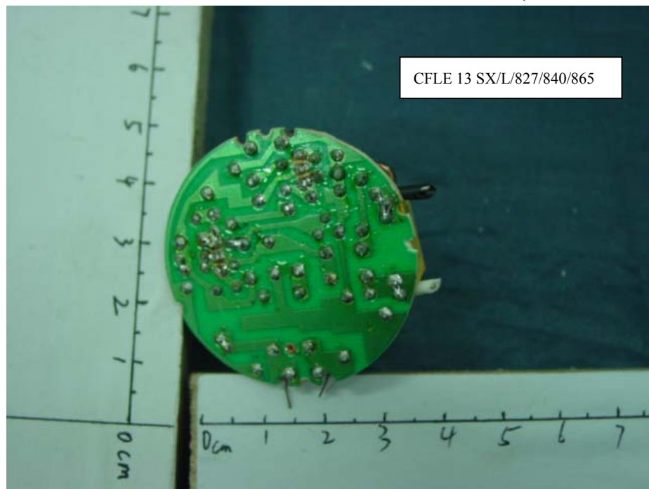
FIGURE 12 Energy Saving Lamp Main Board (Soldered Side)
