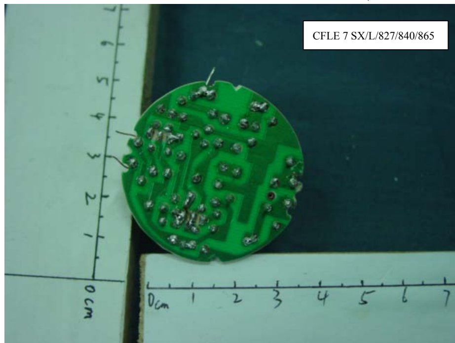
FIGURE 6 Energy Saving Lamp Main Board (Soldered Side)
