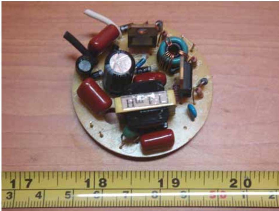
PCB - Front View For CFLE26SX/L/827/840/865
