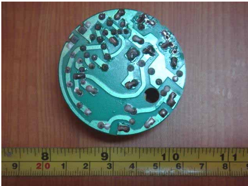
PCB - Back View For CFLE26S/L/827/840/865
