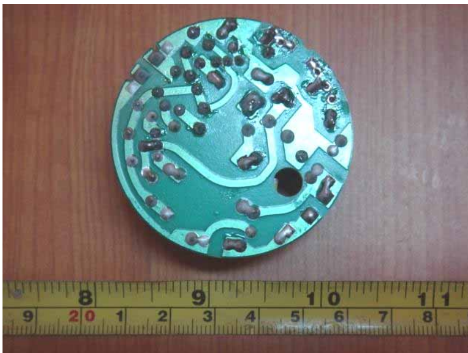
PCB - Back View For CFLE23S/L/827/840/865
