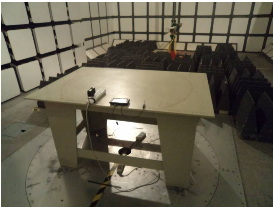
Radiated Emissions- Rear View (Running&Data transmitting with USB disk, 1000-6000 MHz)
