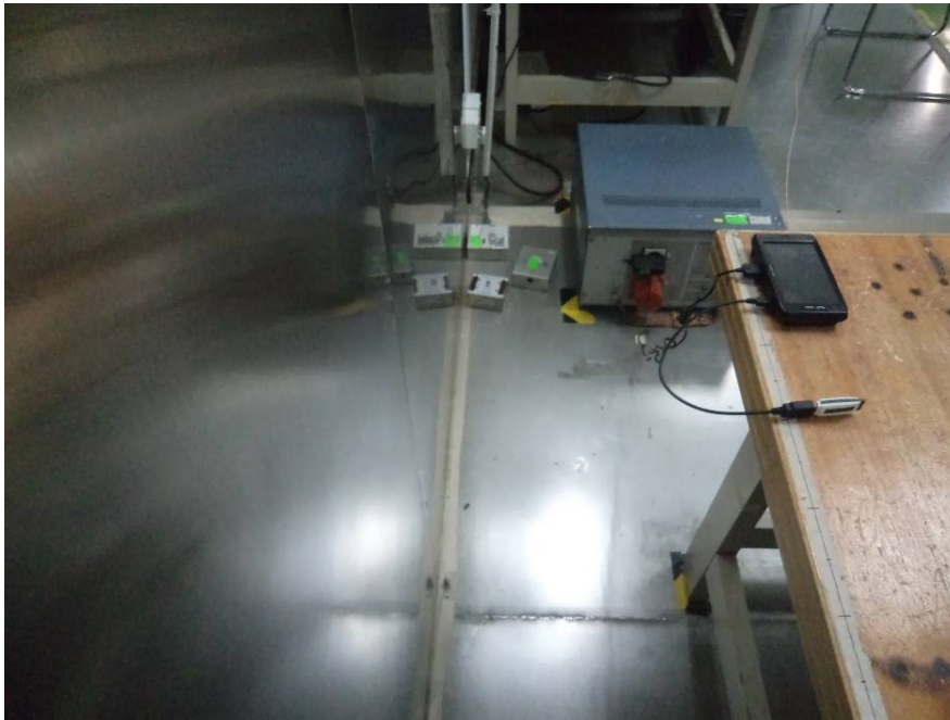
Conducted Emissions - Side View (Running & Data transmitting with USB disk)
