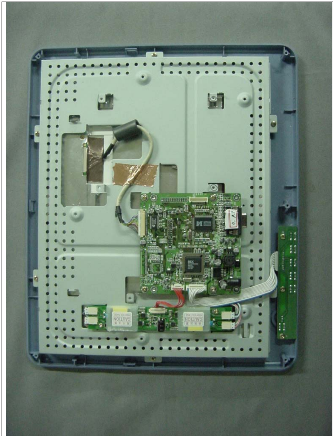
[Inside View after opening Shield Case for Inverter manufactured by FRONTEK CO., LTD.]
