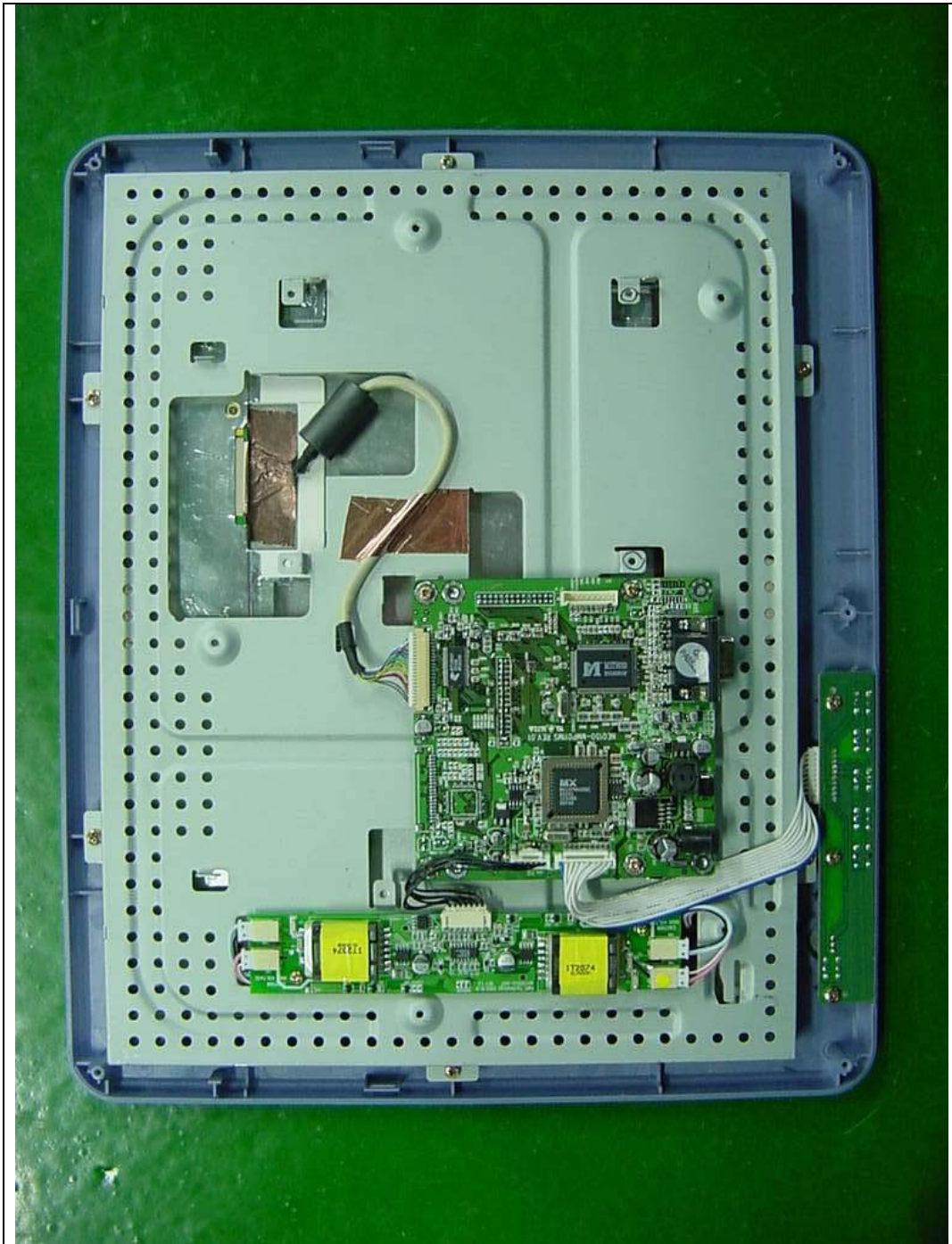
[Inside View after opening Shield Case for Inverter manufactured by GMS Technology ]
