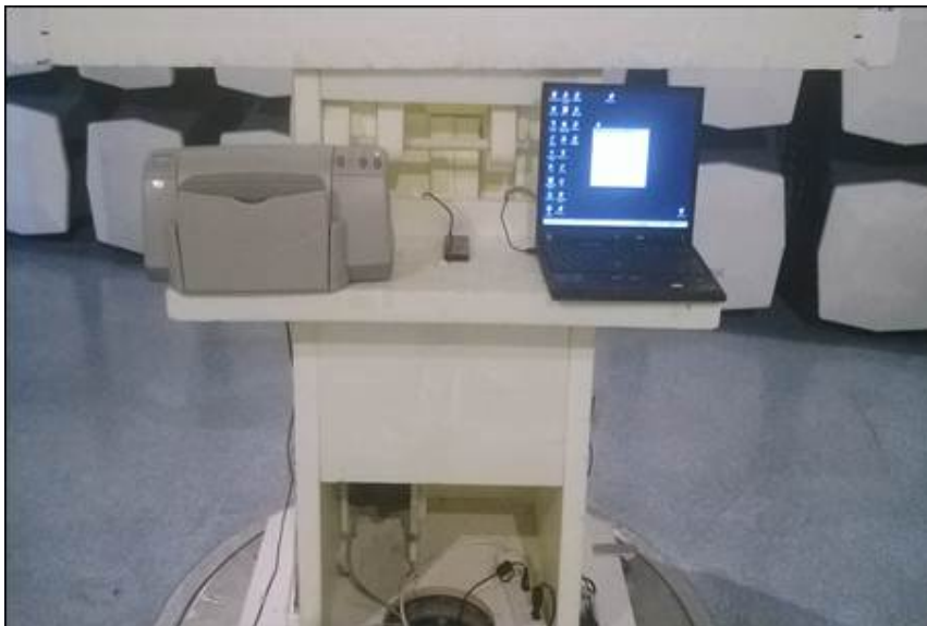
Picture 3. FCC Part 15B Radiated emissions, computer peripherals
