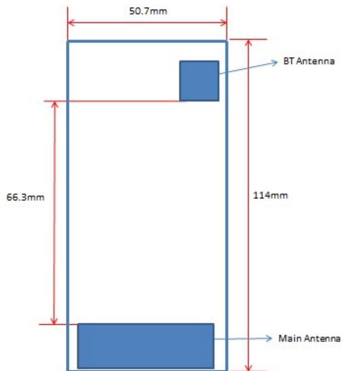
Phone Dimension and Distance Between Main antenna and BT Antenna
