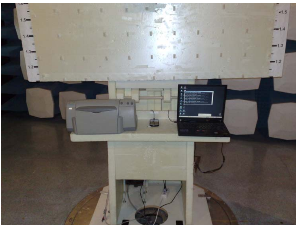
Picture 3. FCC Part 15B Radiated emissions, computer peripherals
