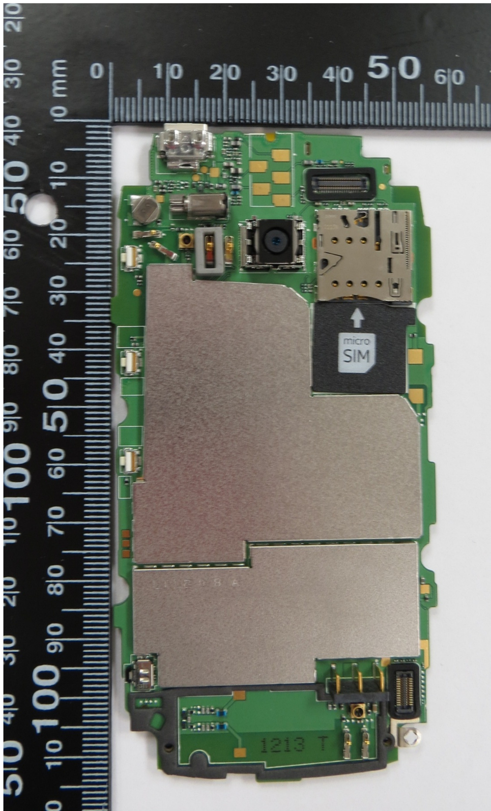
Exhibit 9: Internal Photographs
