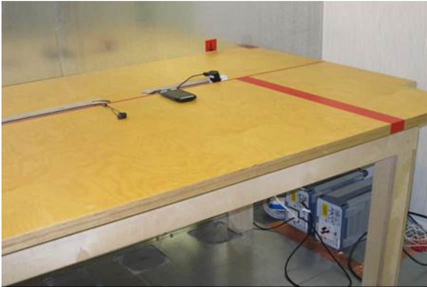
Picture 3. FCC Part 15C AC powerline conducted emissions
