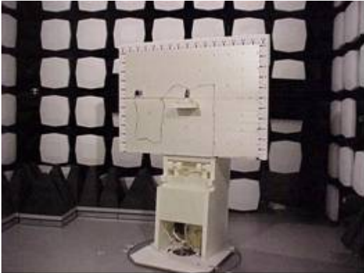
Picture 3. FCC Part 15B Radiated emissions
