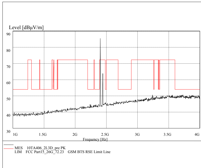
Fig. 45 Radiated emission: 8DPSK, Channel 0, 1 GHz - 4 GHz
