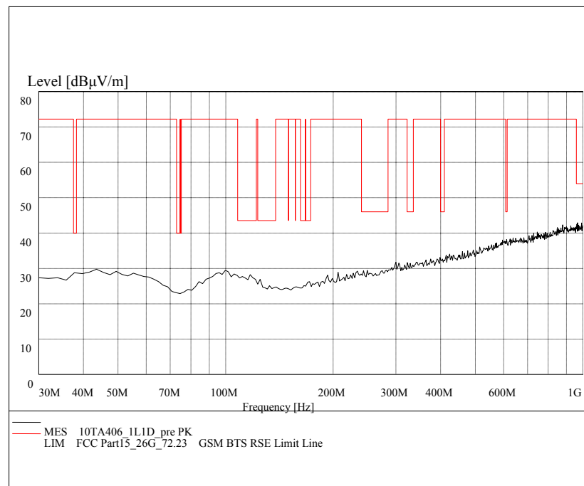
Fig. 22 Radiated emission: GFSK, Channel 0, 30 MHz - 1 GHz
