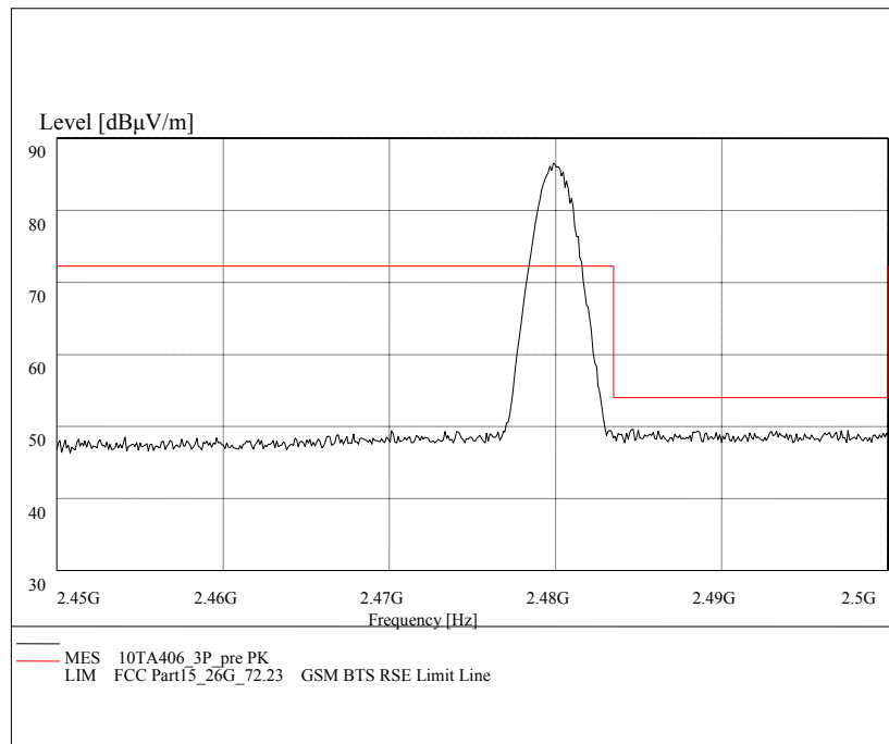
Fig. 53 Radiated emission (Power): 8DPSK, 2.45GHz - 2.5GHz
