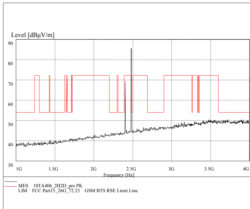
Fig. 40 Radiated emission: \pi/4 DQPSK, Channel 78, 1 GHz - 4 GHz
