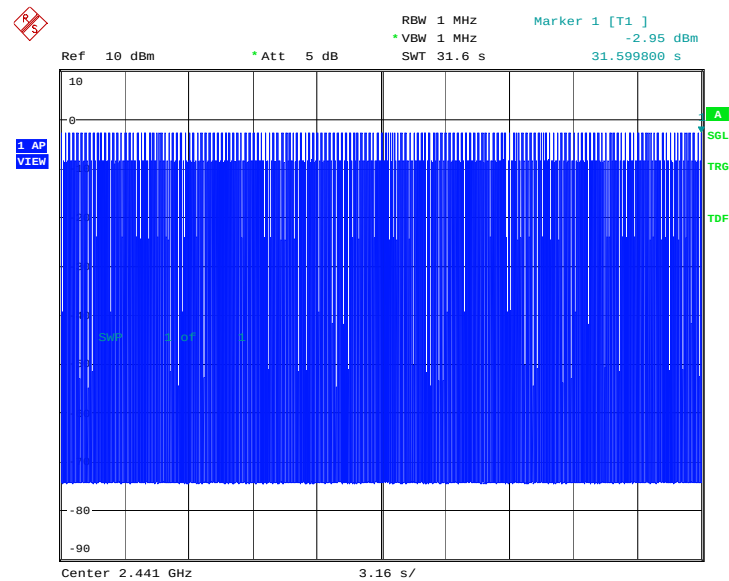
Fig. 61 Time of occupancy (Dwell Time): Channel 39, Packet 2-DH1
