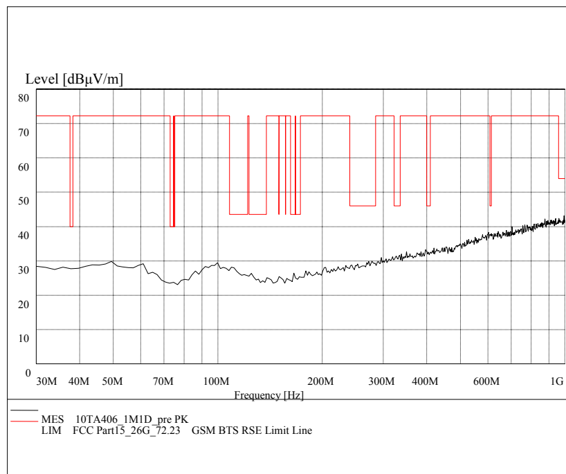
Fig. 25 Radiated emission: GFSK, Channel 39, 30 MHz - 1 GHz
