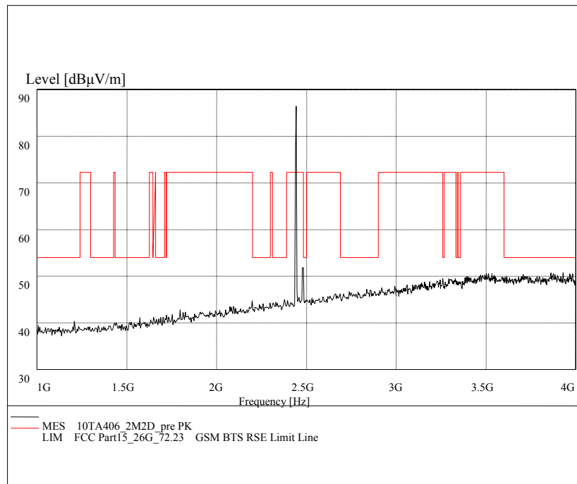
Fig. 37 Radiated emission: \pi/4 DQPSK, Channel 39, 1 GHz - 4 GHz
