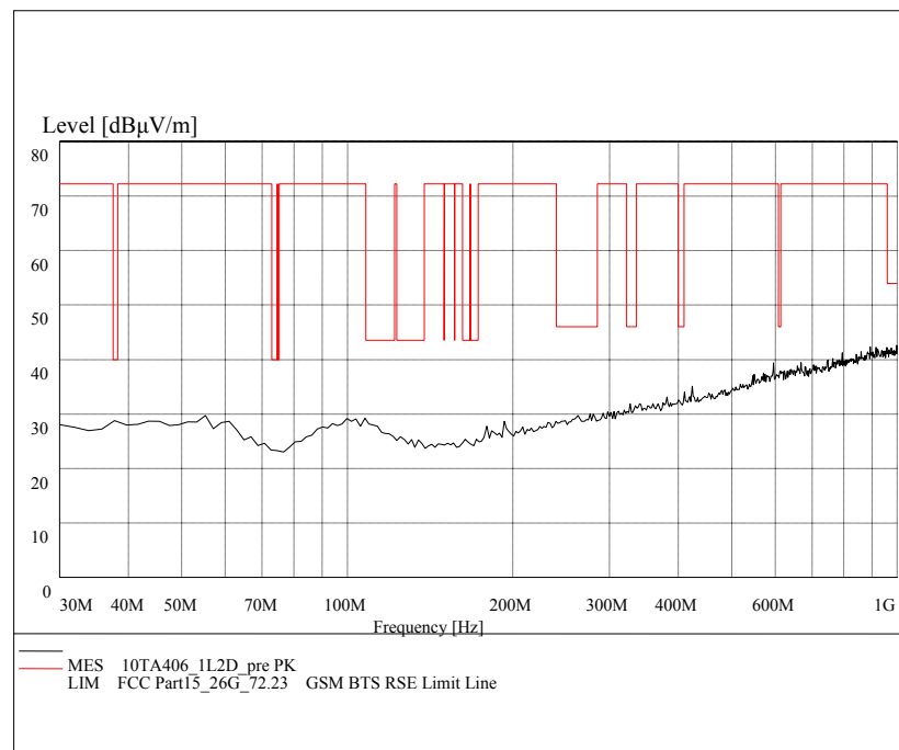
Fig. 33 Radiated emission: \pi/4 DQPSK, Channel 0, 30 MHz - 1 GHz
