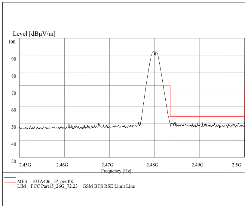
Fig. 31 Radiated emission (Power): GFSK, 2.45GHz - 2.5GHz
