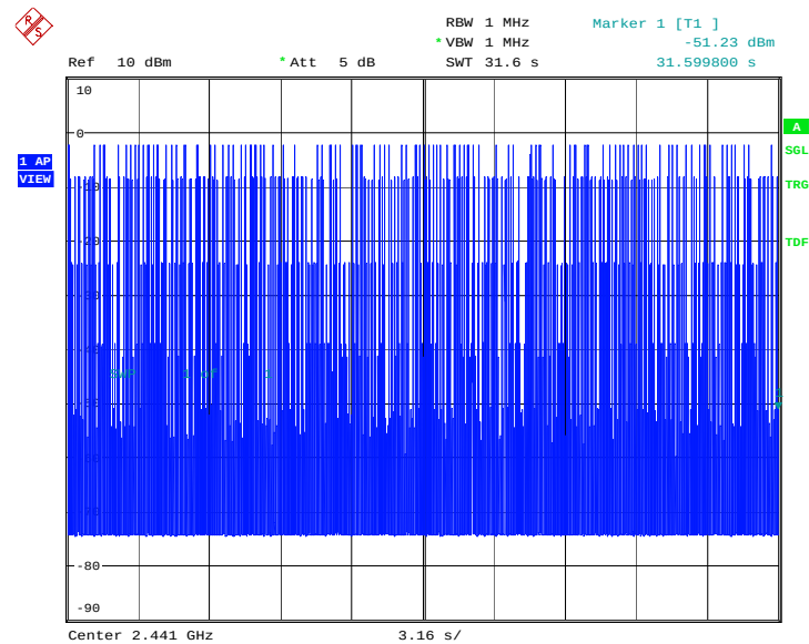
Fig. 69 Time of occupancy (Dwell Time): Channel 39, Packet 3-DH3
