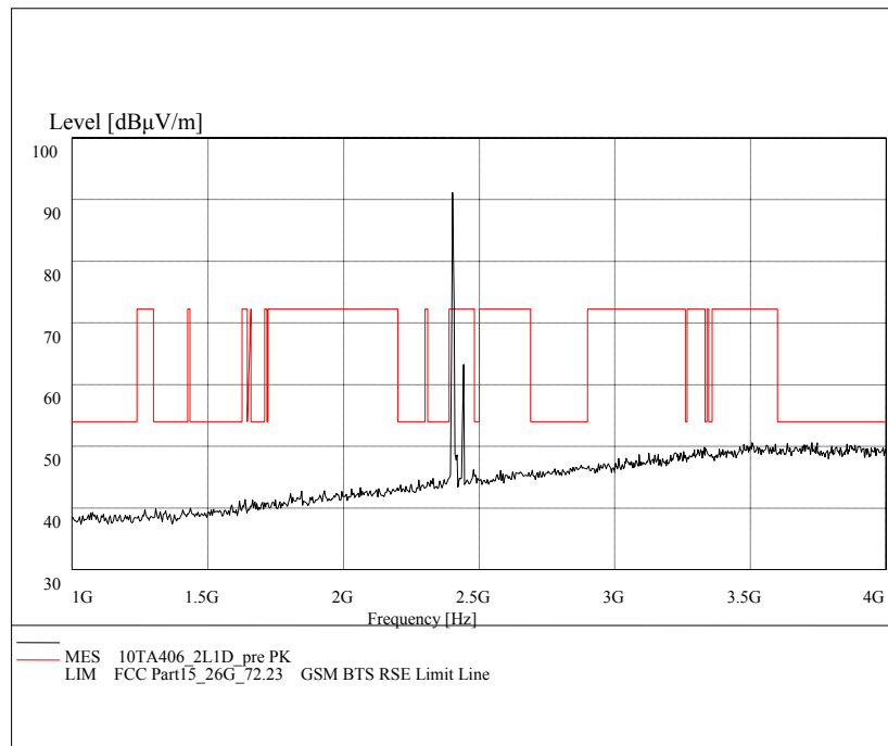
Fig. 23 Radiated emission: GFSK, Channel 0, 1 GHz - 4 GHz
