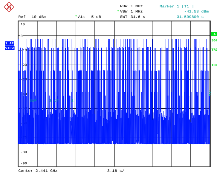
Fig. 71 Time of occupancy (Dwell Time): Channel 39, Packet 3-DH5
