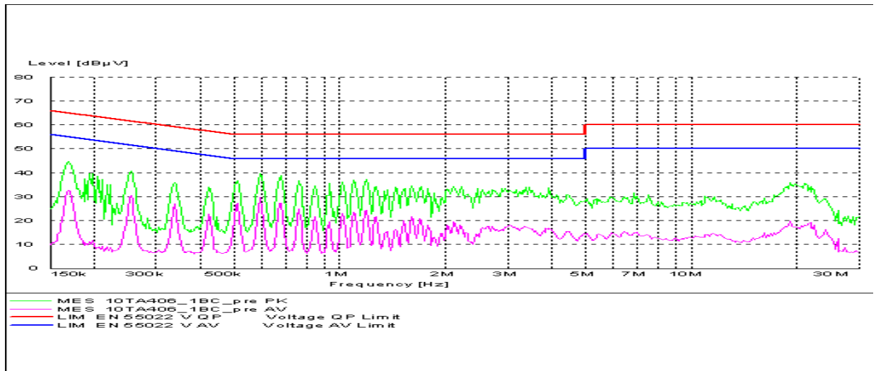
Fig. 91 AC Powerline Conducted Emission with charger-TX mode
