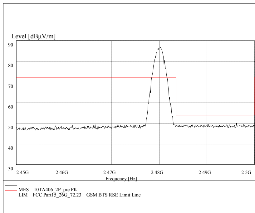
Fig. 42 Radiated emission (Power): \pi/4 DQPSK, 2.45GHz - 2.5GHz
