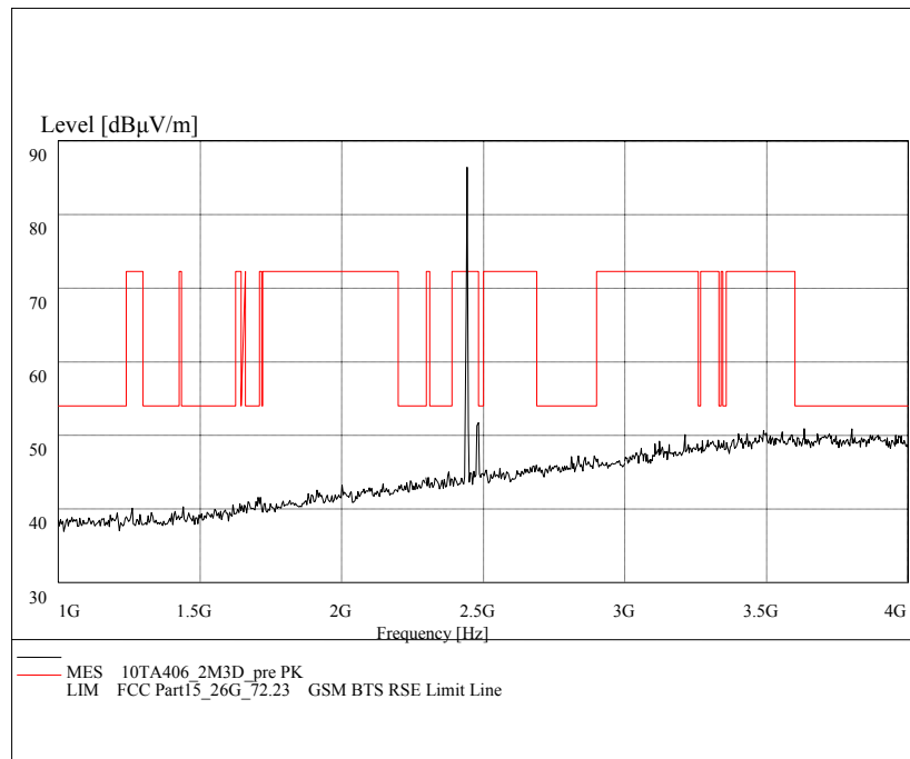
Fig. 48 Radiated emission: 8DPSK, Channel 39, 1 GHz - 4 GHz
