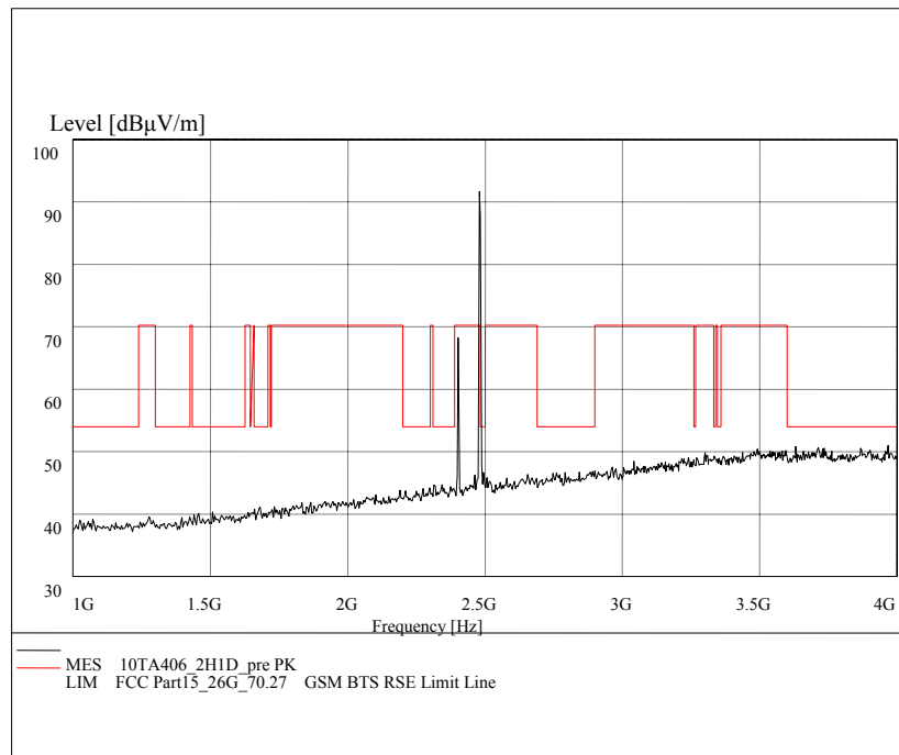
Fig. 29 Radiated emission: GFSK, Channel 78, 1 GHz - 4 GHz
