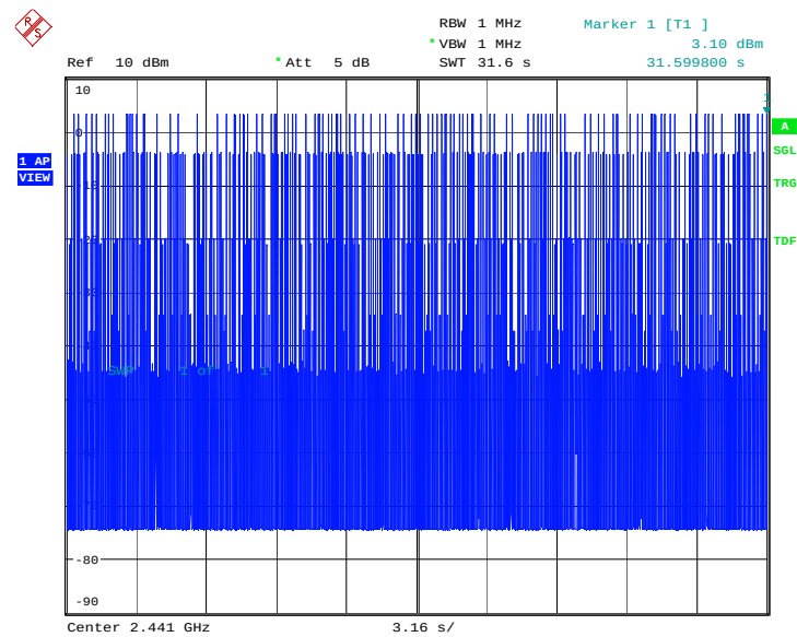
Fig. 57 Time of occupancy (Dwell Time): Channel 39, Packet DH3
