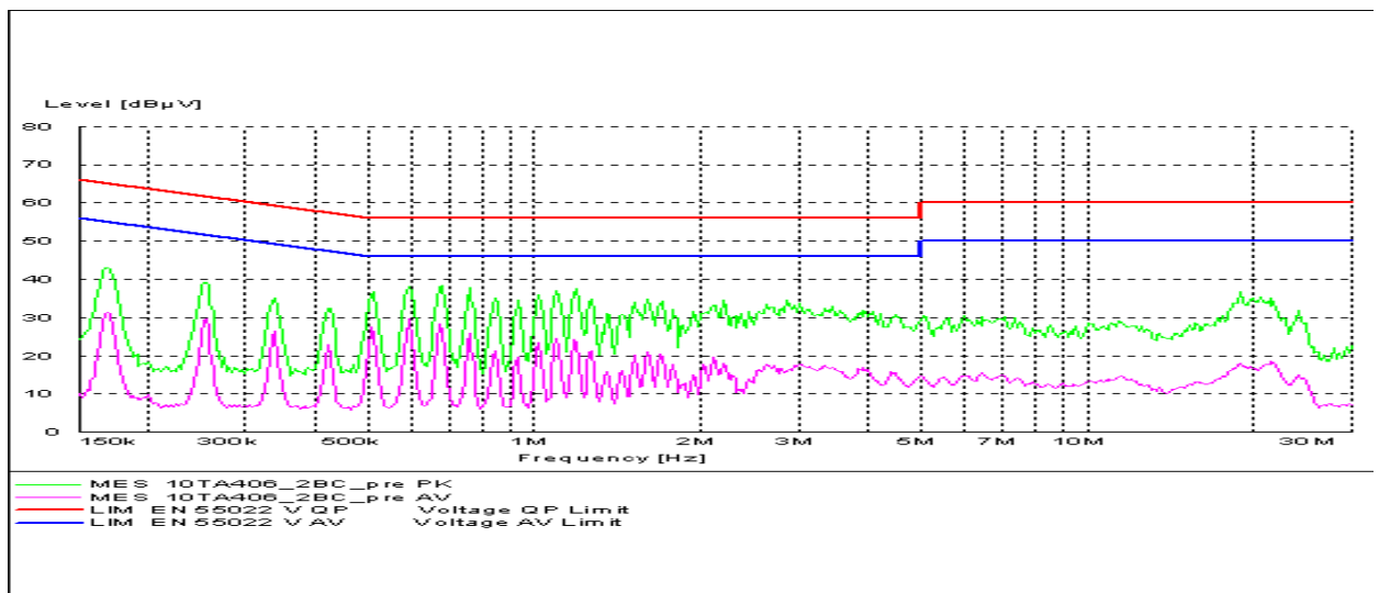
Fig. 92 AC Powerline Conducted Emission with charger-Idle mode
