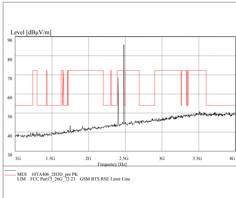
Fig. 51 Radiated emission: 8DPSK, Channel 78, 1 GHz - 4 GHz
