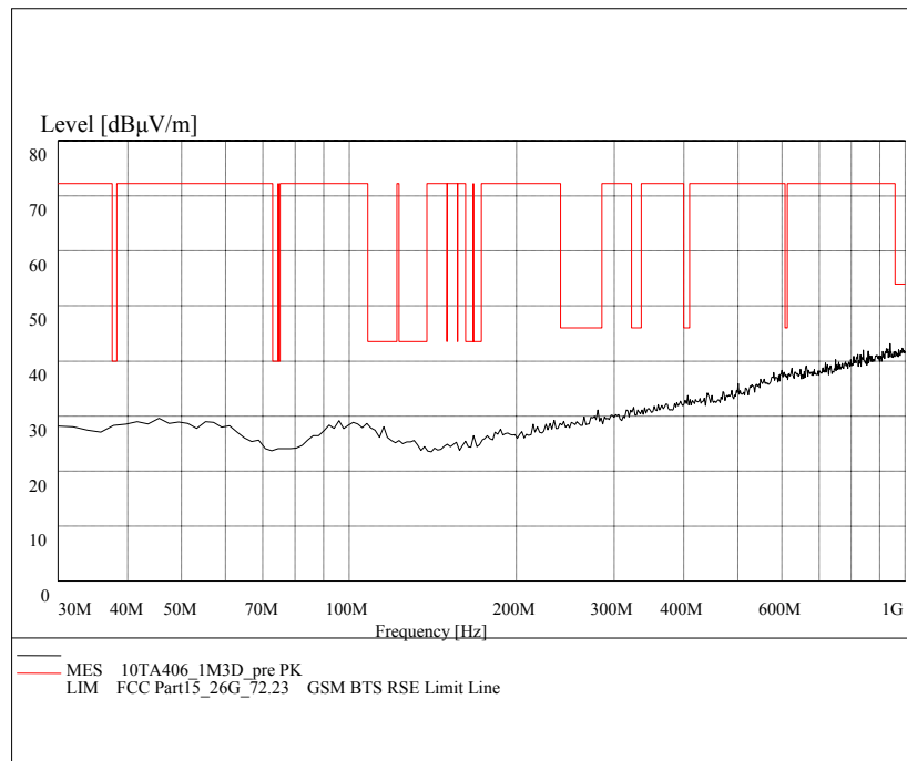
Fig. 47 Radiated emission: 8DPSK, Channel 39, 30 MHz - 1 GHz
