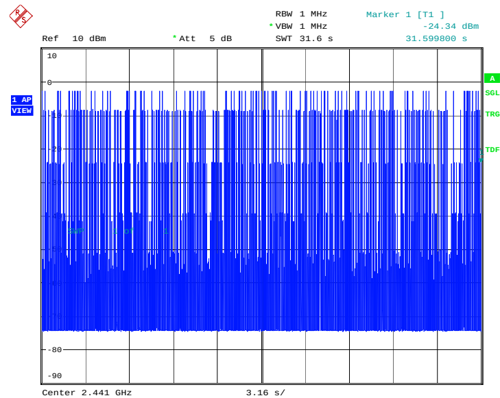
Fig. 63 Time of occupancy (Dwell Time): Channel 39, Packet 2-DH3
