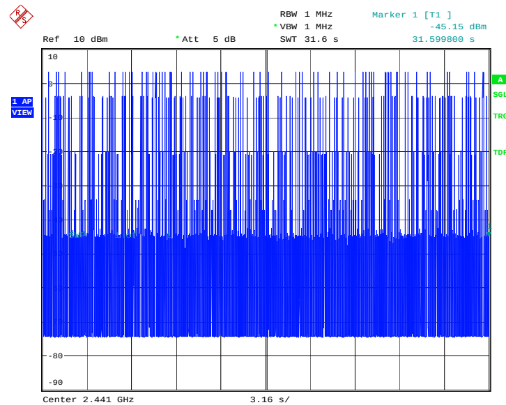
Fig. 59 Time of occupancy (Dwell Time): Channel 39, Packet DH5
