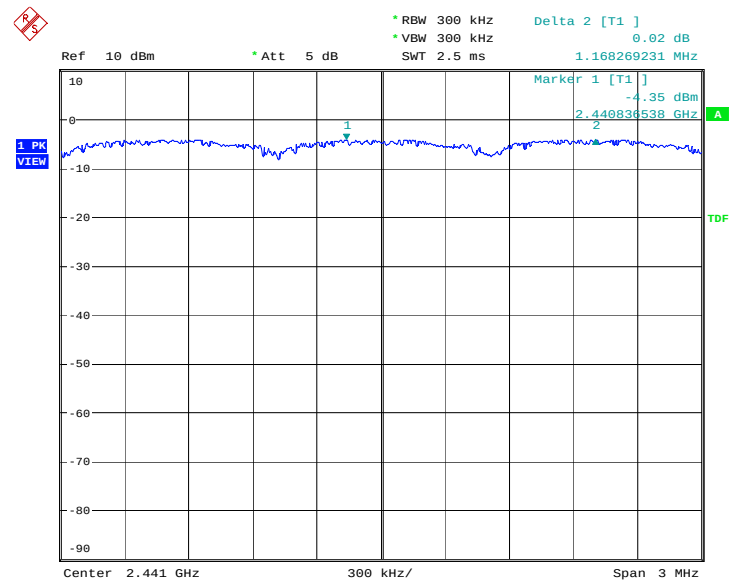
Fig. 83 Carrier frequency separation measurement: \pi/4 DQPSK, Channel 39
