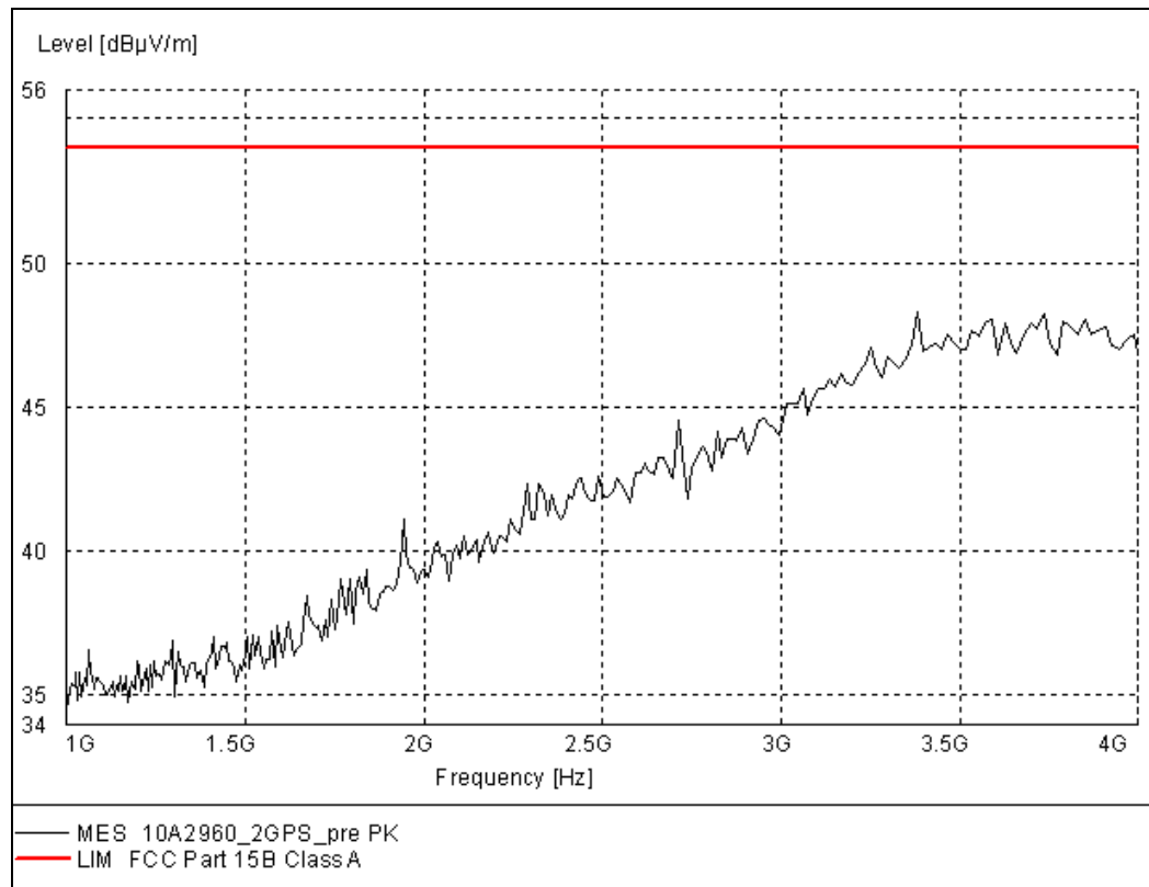
Figure A.5 Radiated Emission from 1GHz to 4GHz
