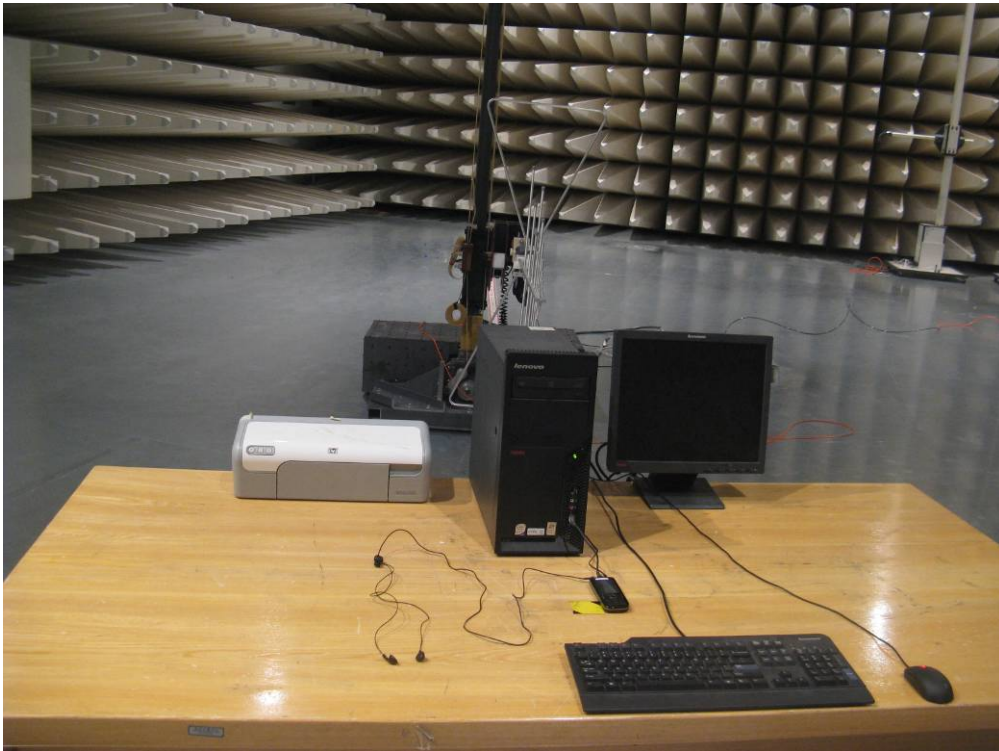
Radiated Emission- Data Transferring
