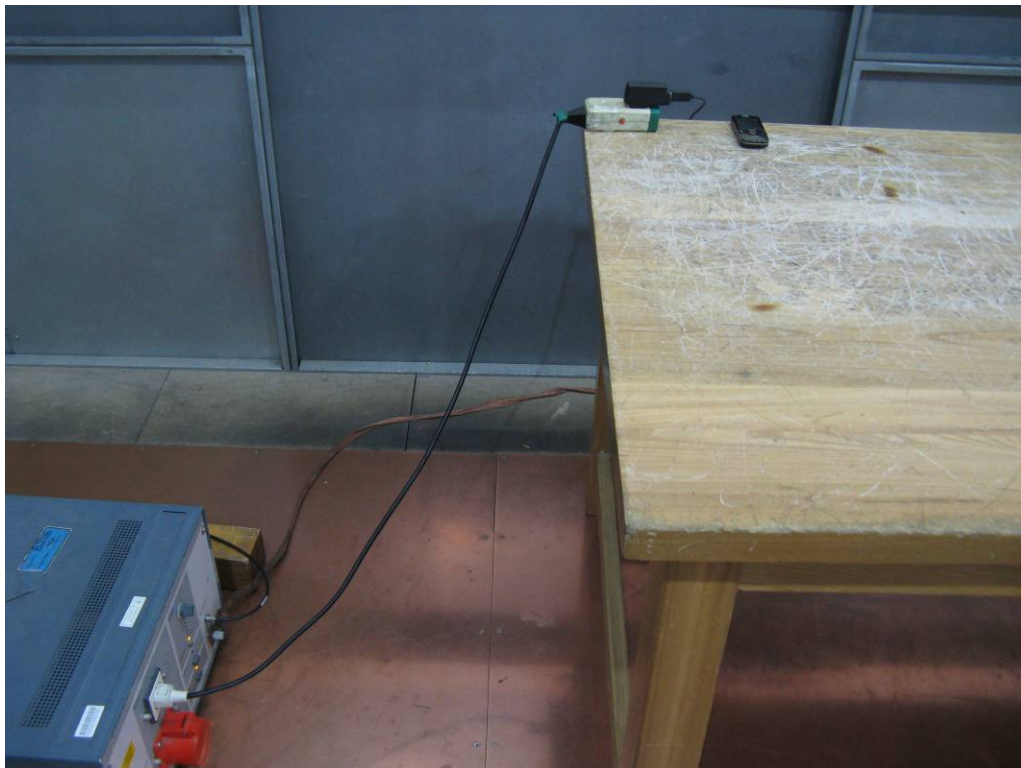
Conducted Emission
