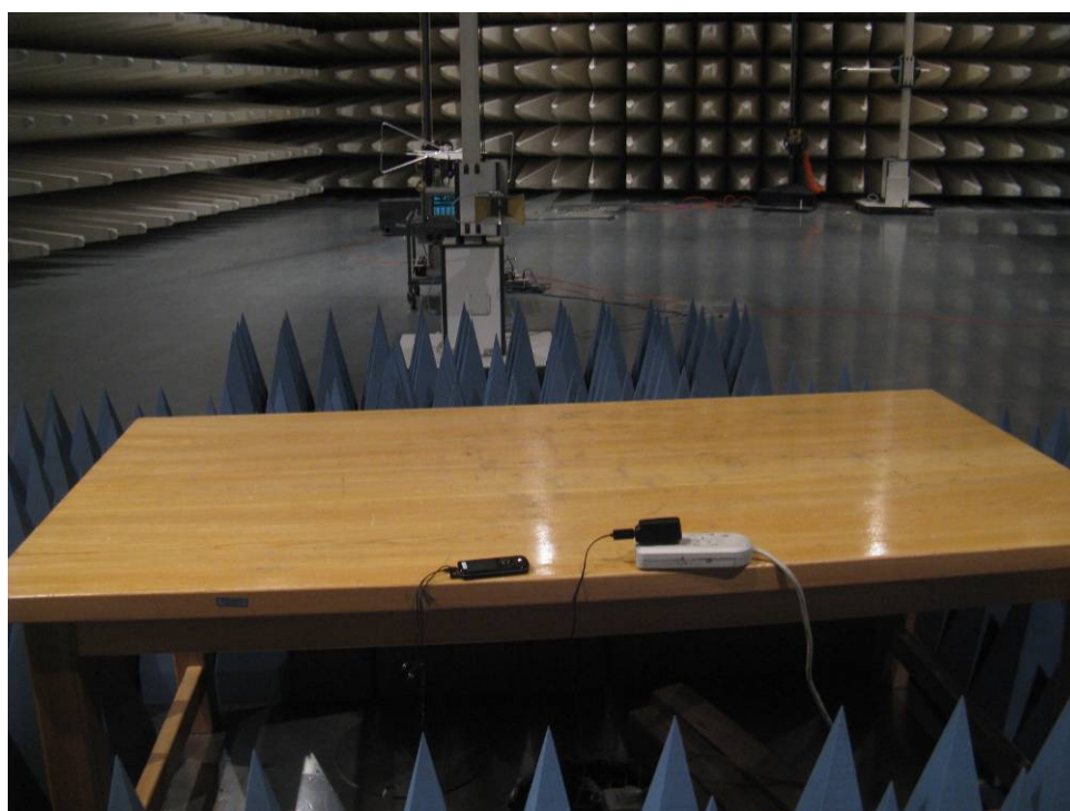
Radiated Emission- GPS(Above 1GHz)
