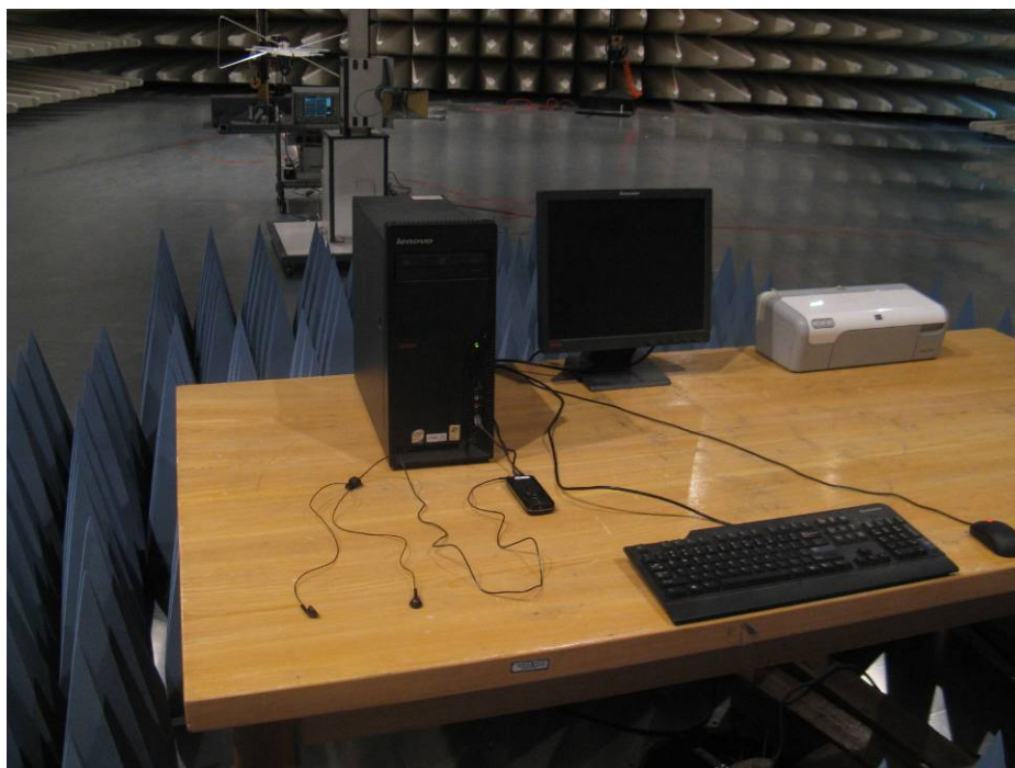
Radiated Emission - Data Transferring (Above 1GHz)
