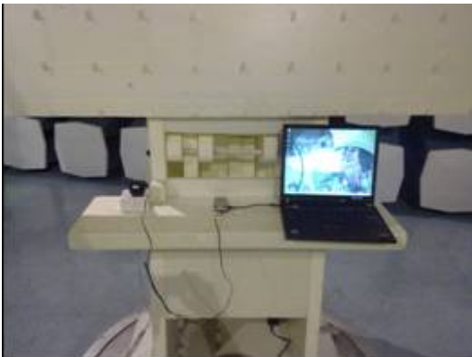
Picture 2. FCC Part 15B Radiated emissions
