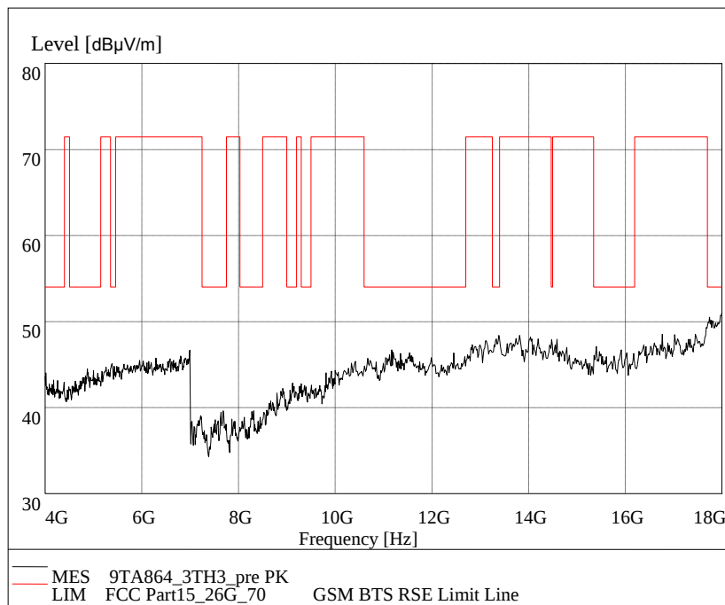
Fig. 70 Radiated emission: 8DPSK, Channel 78, 4 GHz - 18 GHz
