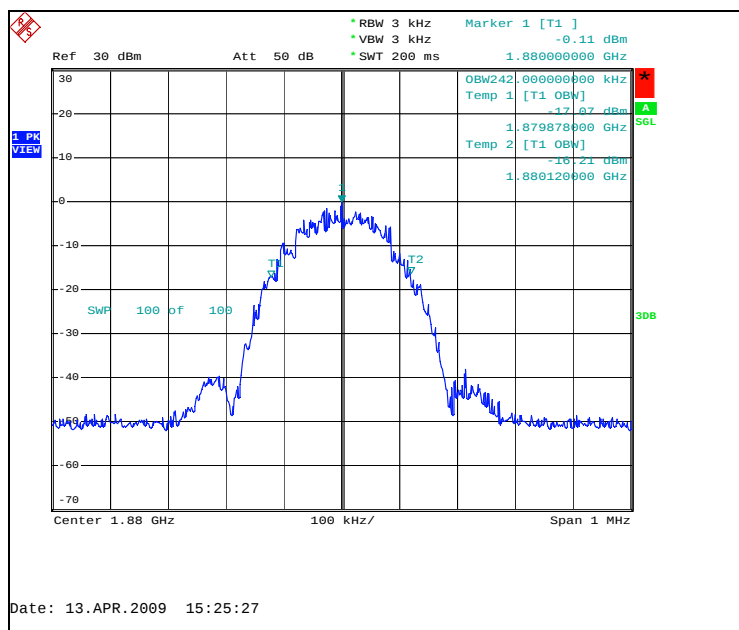
EGPRS mode, channel 661 / 1880.0 MHz
