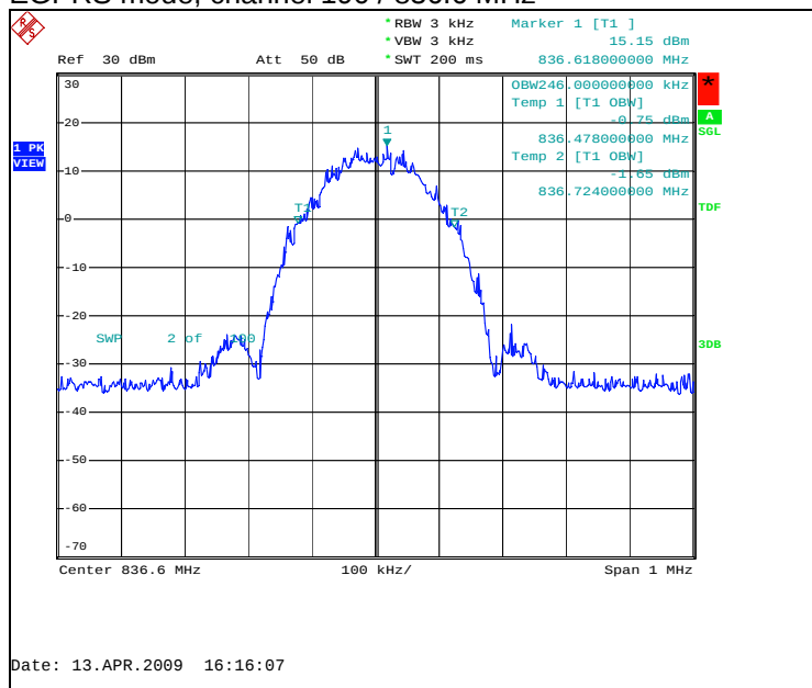
EGPRS mode, channel 190 / 836.6 MHz
