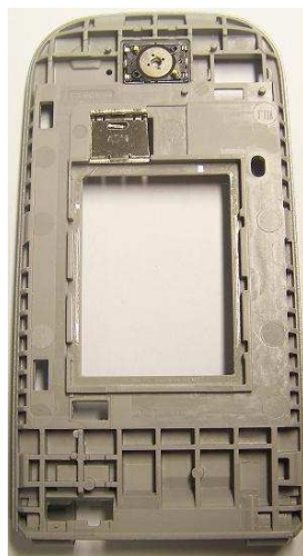
B-cover bottom view
