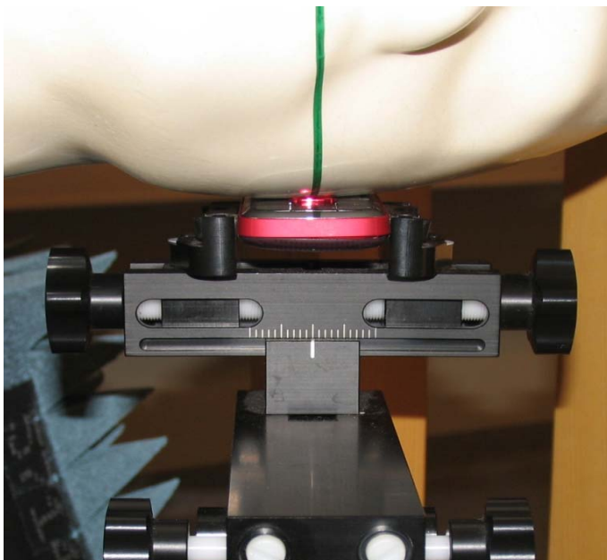
Photo of the device in “cheek” position
