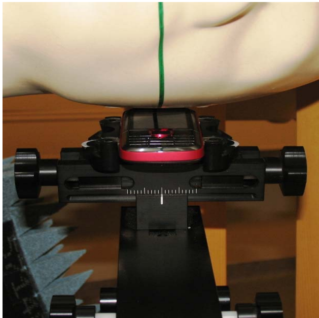
Photo of the device in “tilt” position
