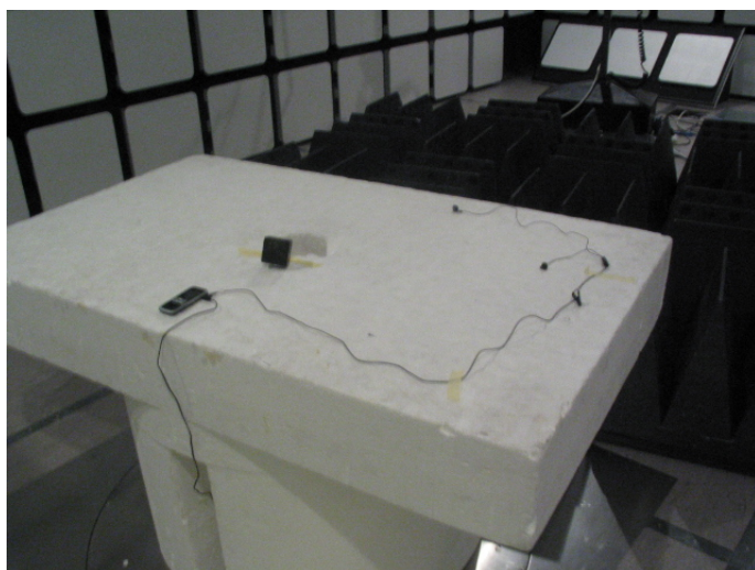
Picture 2 Radiated emission measurement GSM RX / Bluetooth TX
