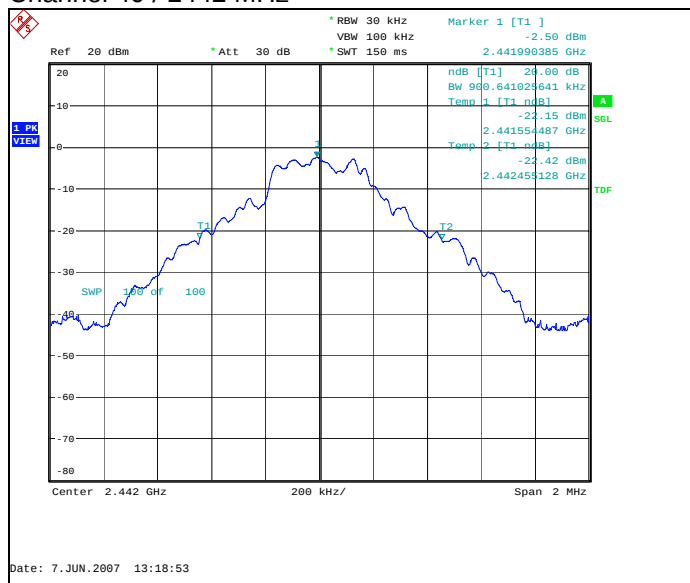
Channel 40 / 2442 MHz
