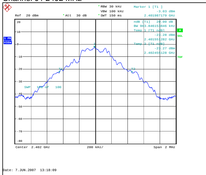
Channel 0 / 2402 MHz
