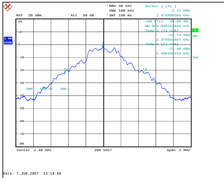
Channel 78 / 2480 MHz
