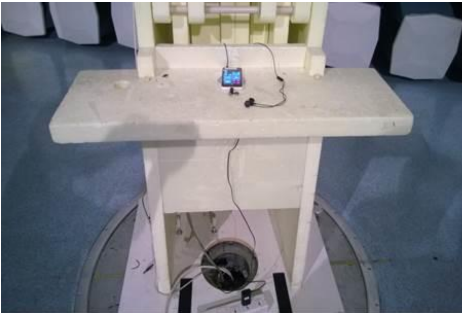
Picture 2. FCC Part 15B Radiated emissions
