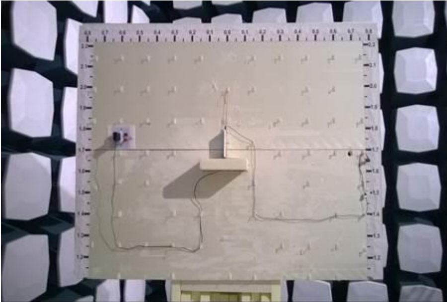
Picture 1. FCC Part 15C Radiated emissions
