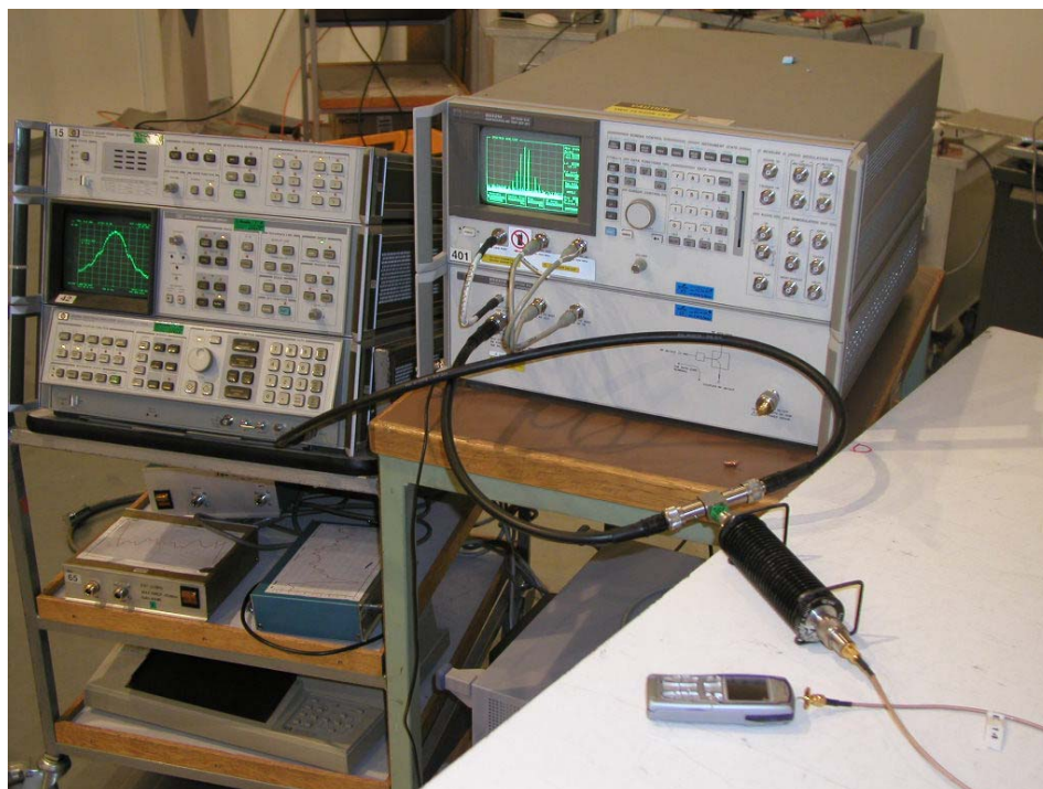
Photograph 2. Test setup for conducted power spectrum measurements
