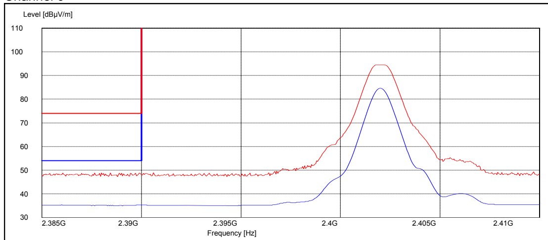
Channel 0
