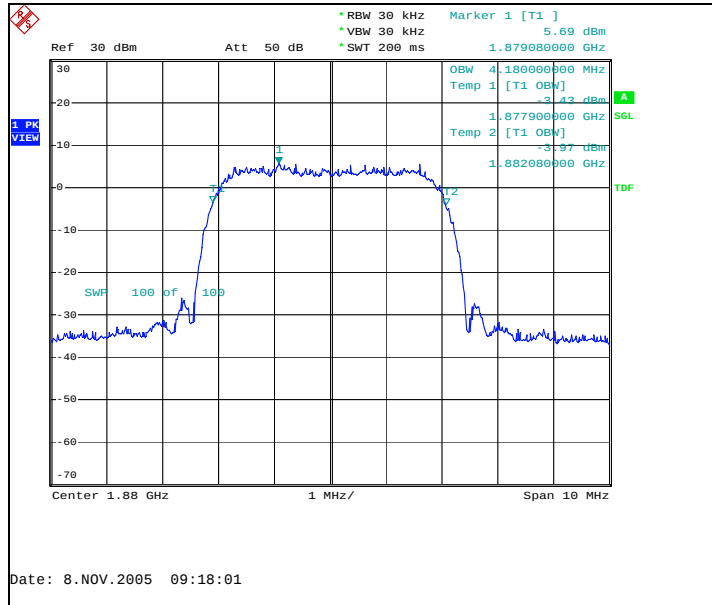
Channel 9400
