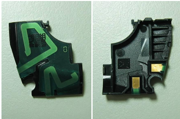
GPS/BT/WLAN Antenna
