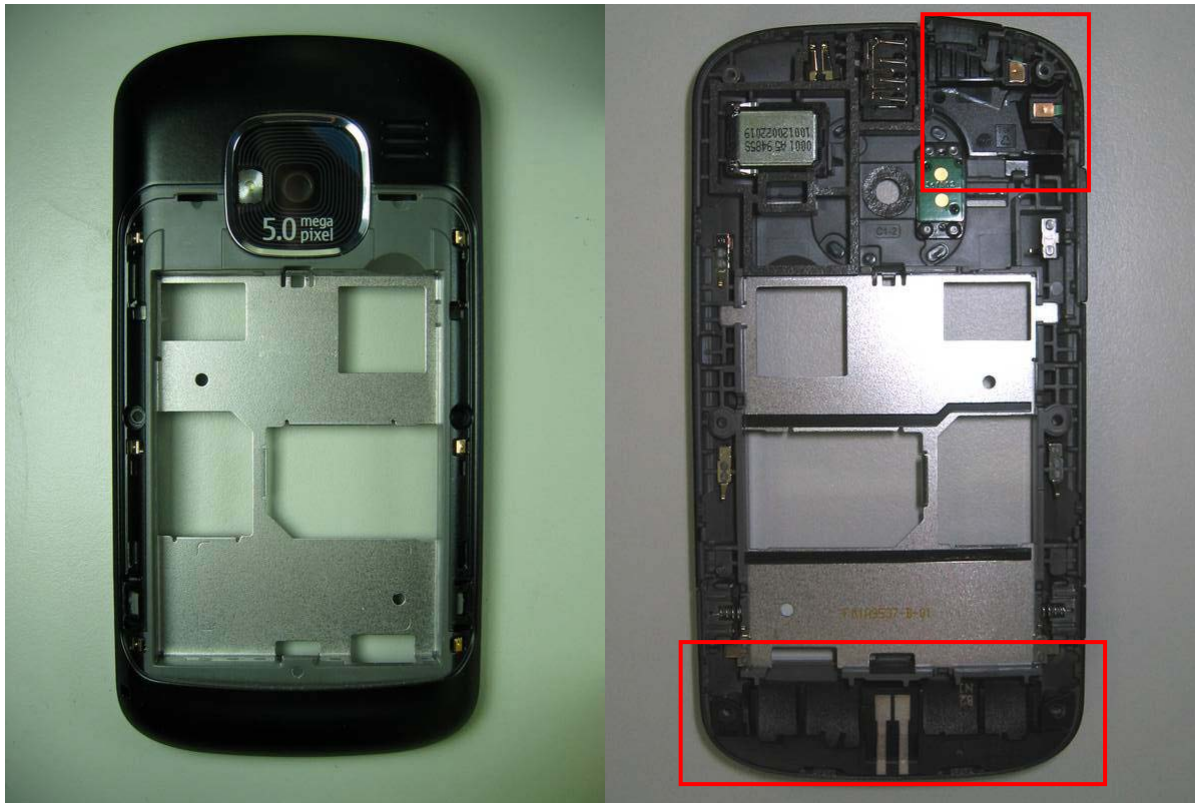
Main Antenna
