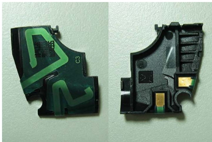
GPS/BT/WLAN Antenna
