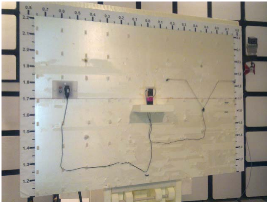
Picture 1. FCC Part 15C Radiated emissions
