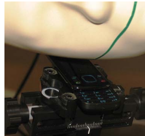
Photo of the device in “tilt” position with slide open
