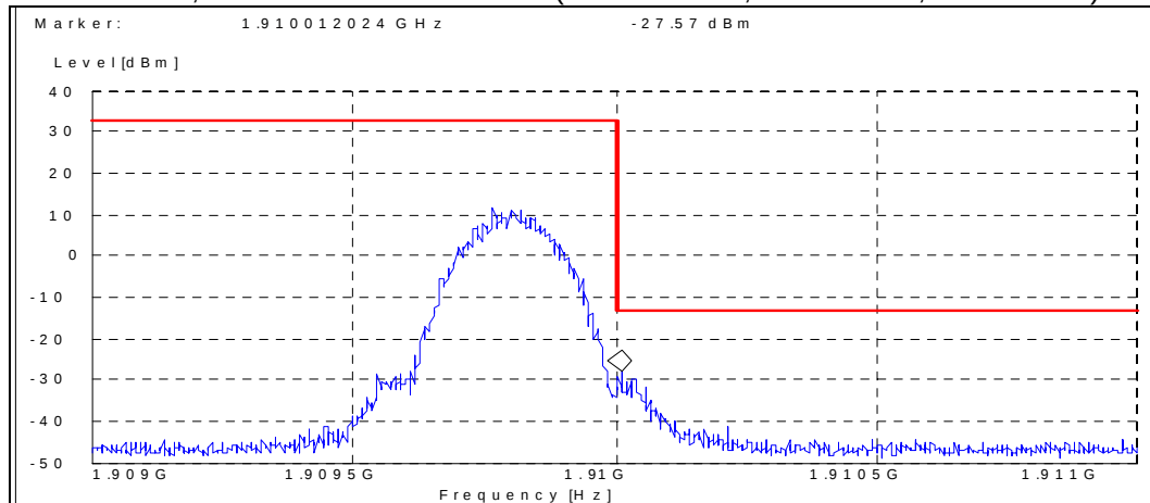
EGPRS mode, channel 810 / 1909.8 MHz (Peak detector, RBW: 3 kHz, VBW: 3 kHz)
