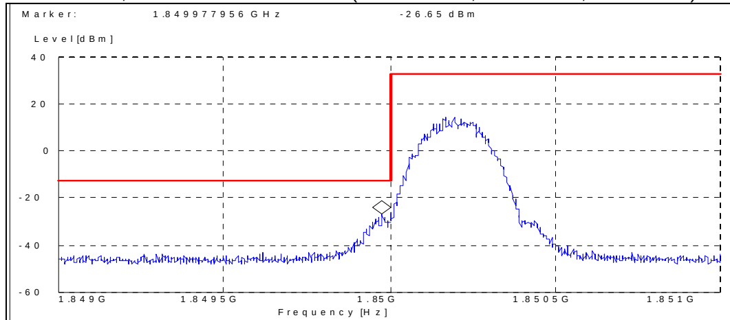
EGPRS mode, channel 512 / 1850.2 MHz (Peak detector, RBW: 3 kHz, VBW: 3 kHz)
